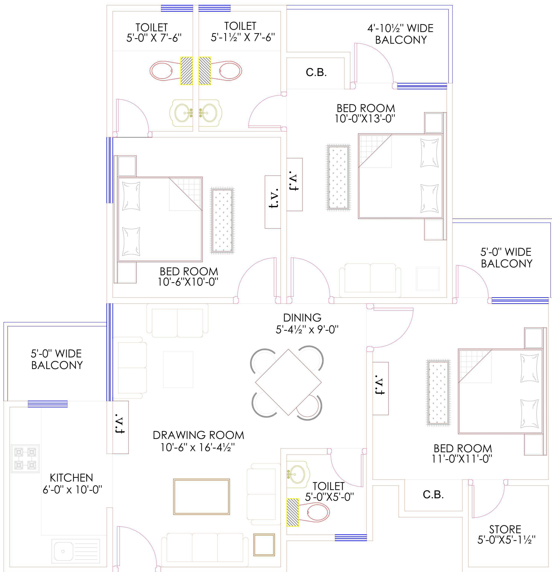
TYPE - 2 3BHK+3TOILET+STORE
