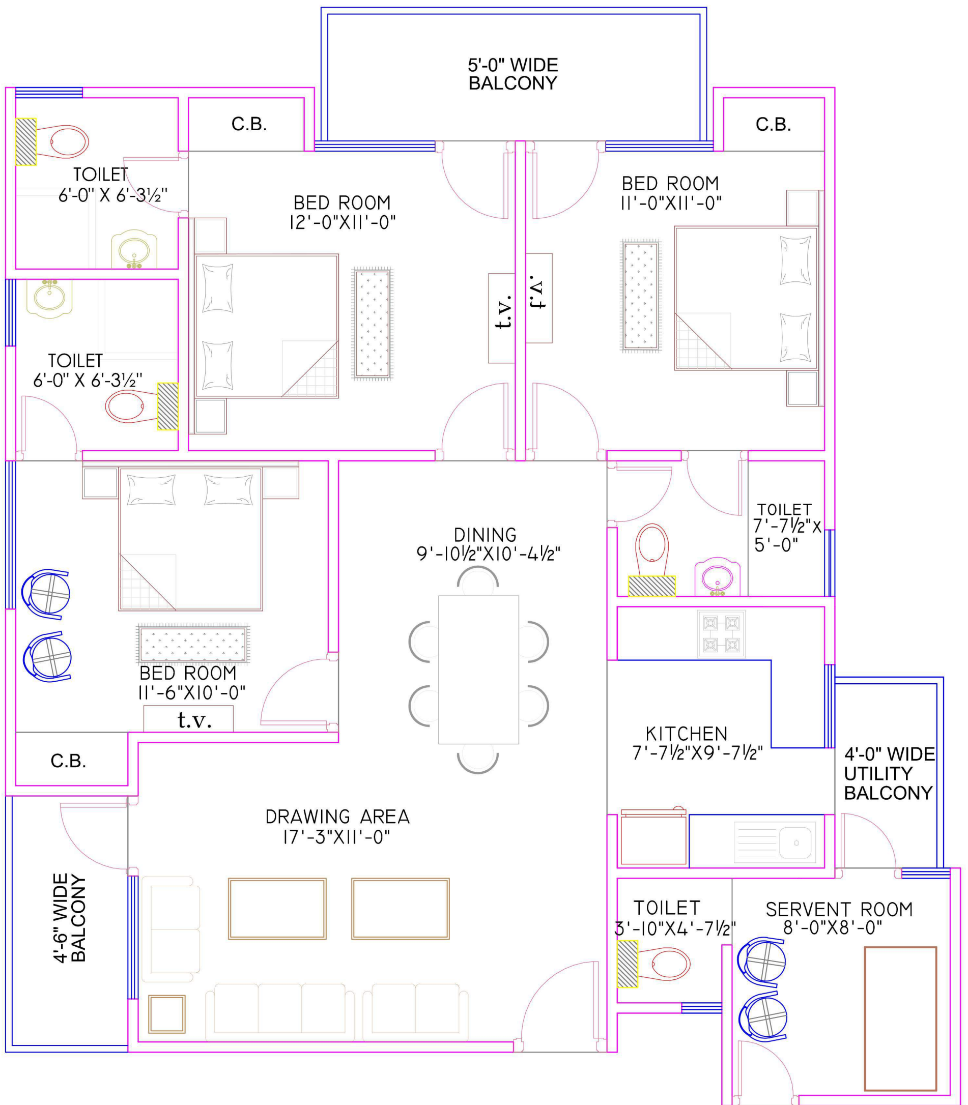
TYPE - 1 3BHK+3TOILET+SERVANT ROOM
