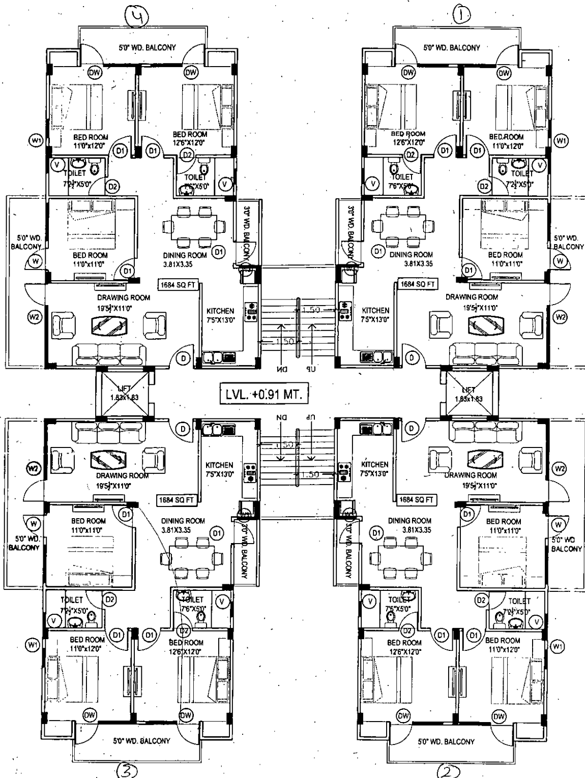
GROUND FLOOR PLAN (RESIDENTIAL ZONE)
