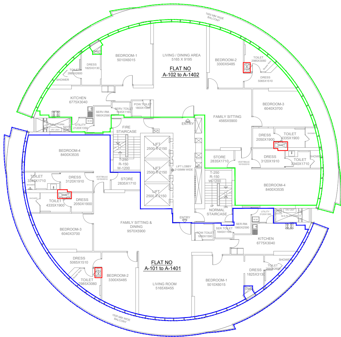
1ST FLOOR TO 14TH FLOOR PLAN
