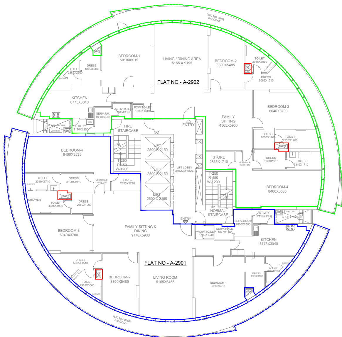
29TH FLOOR PLAN
