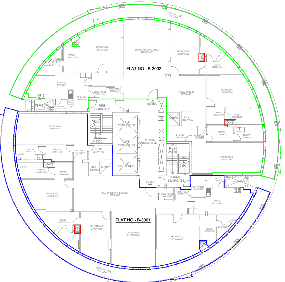
30TH FLOOR PLAN
