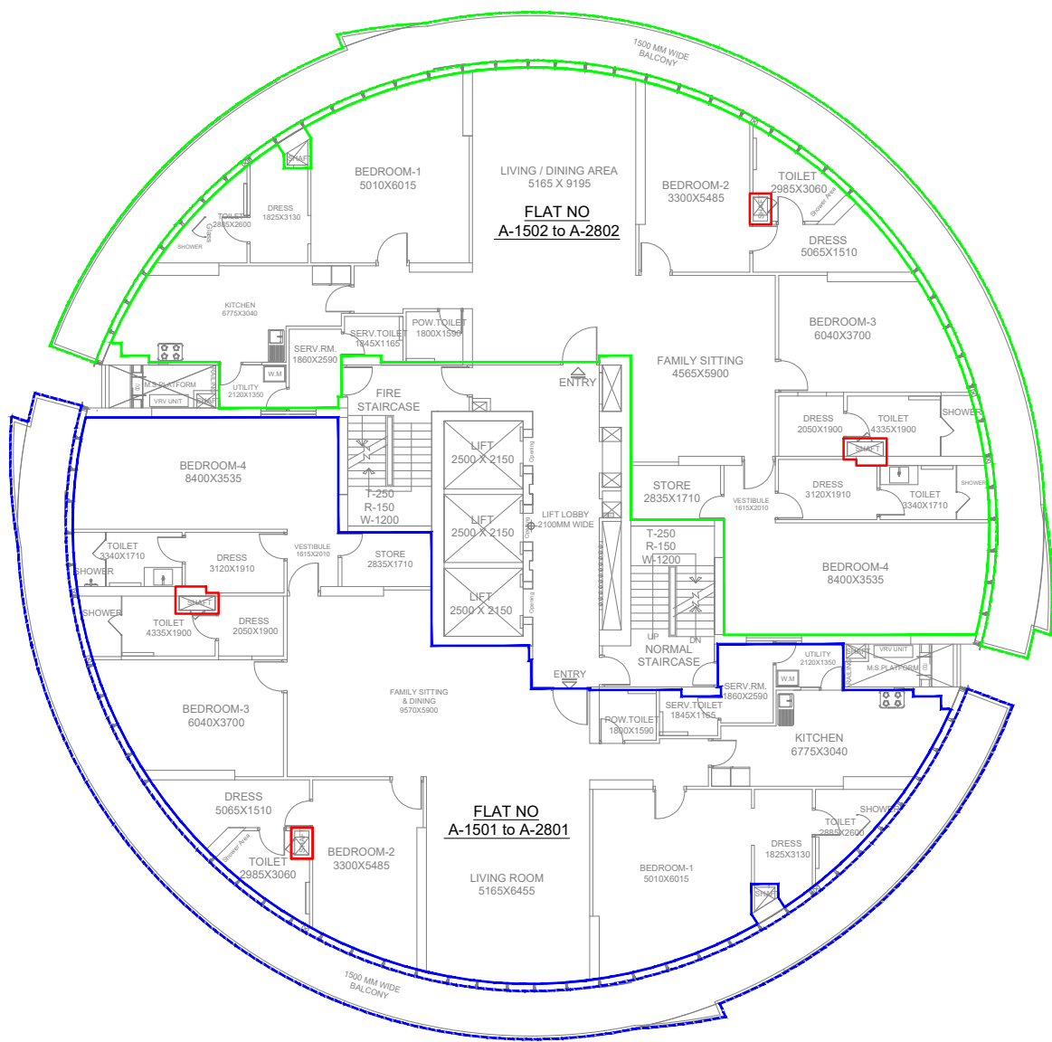
15TH FLOOR TO 28TH FLOOR PLAN
