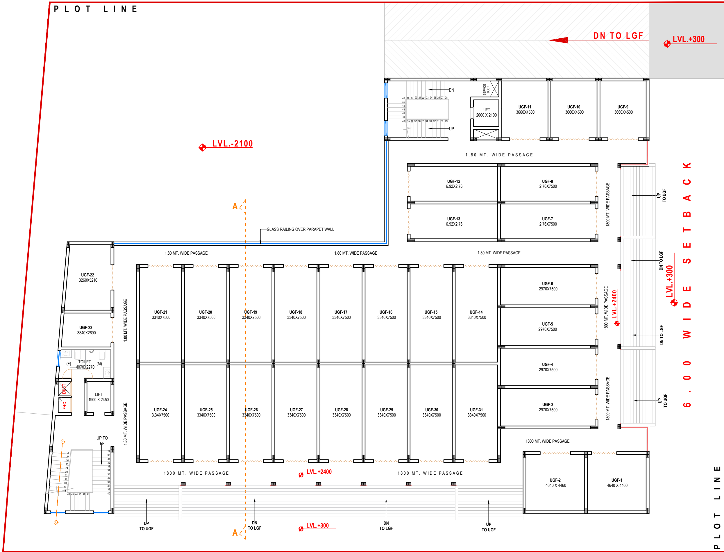
UPPER GROUND FLOOR PLAN
