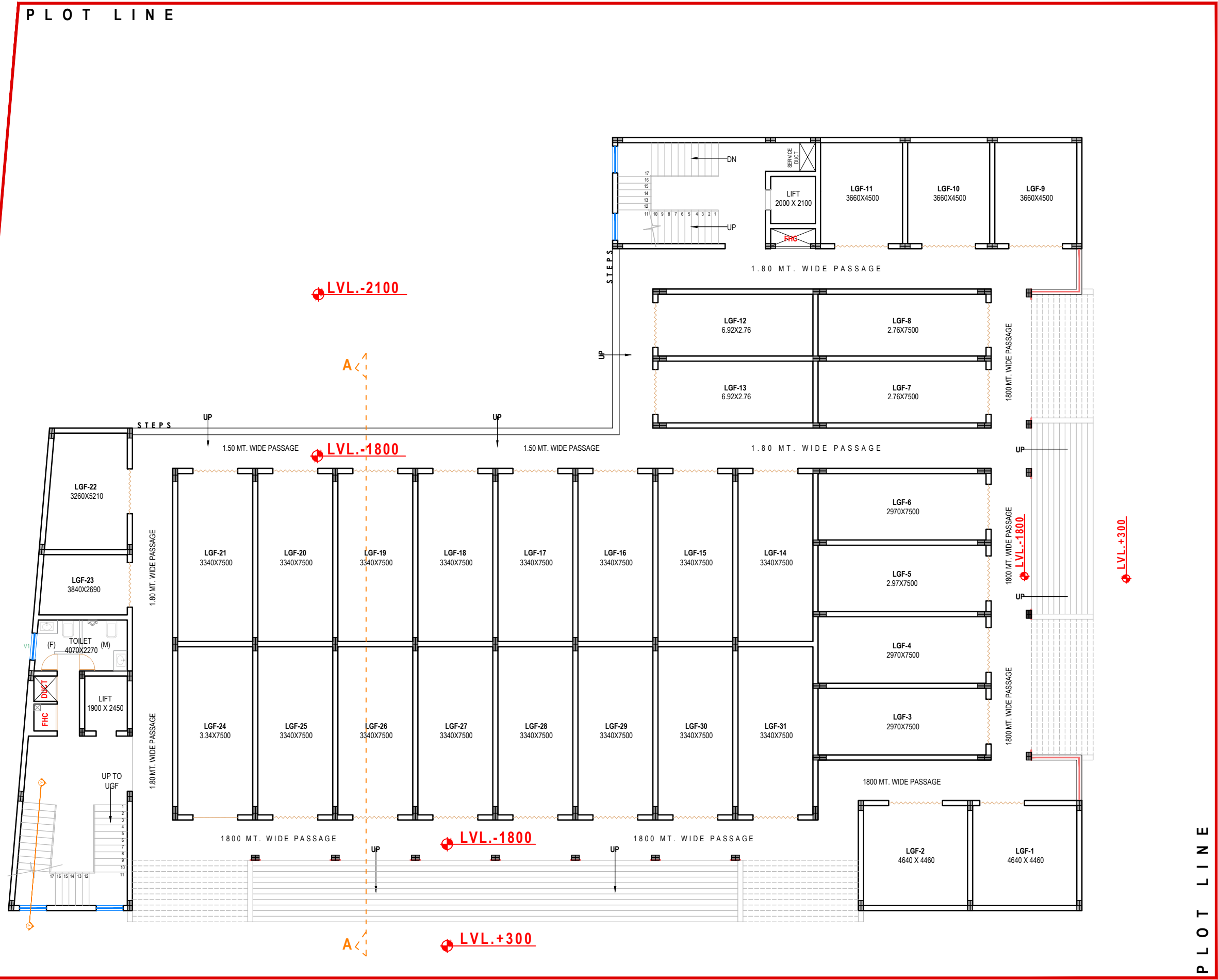
LOWER GROUND FLOOR PLAN
