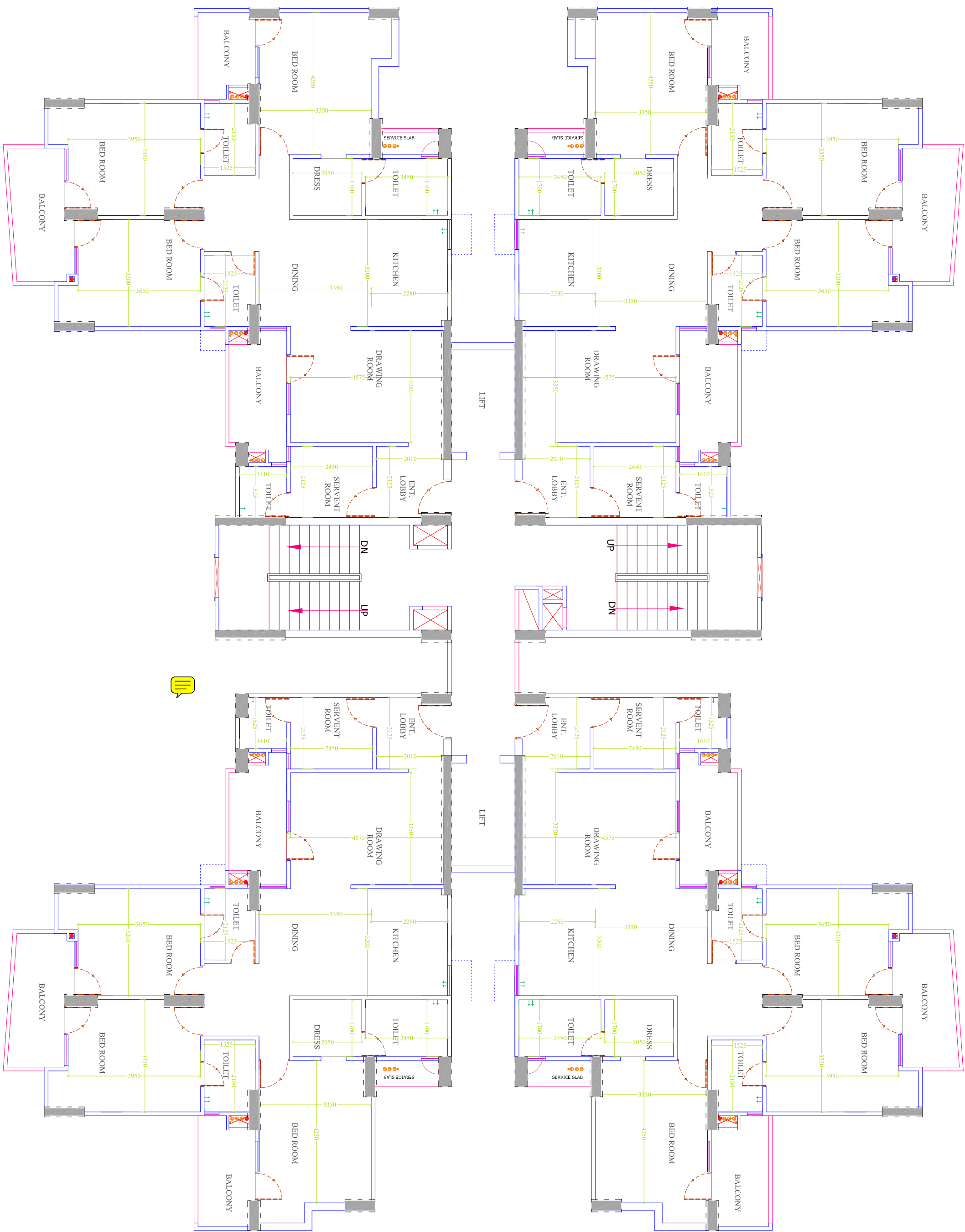
TOWER-F1 TYPICAL FLOOR PLAN
