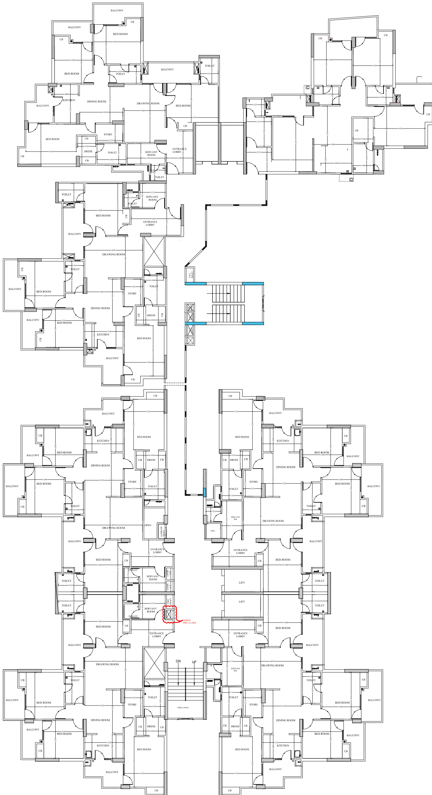
TOWER-G5 TYPICAL FLOOR PLAN
