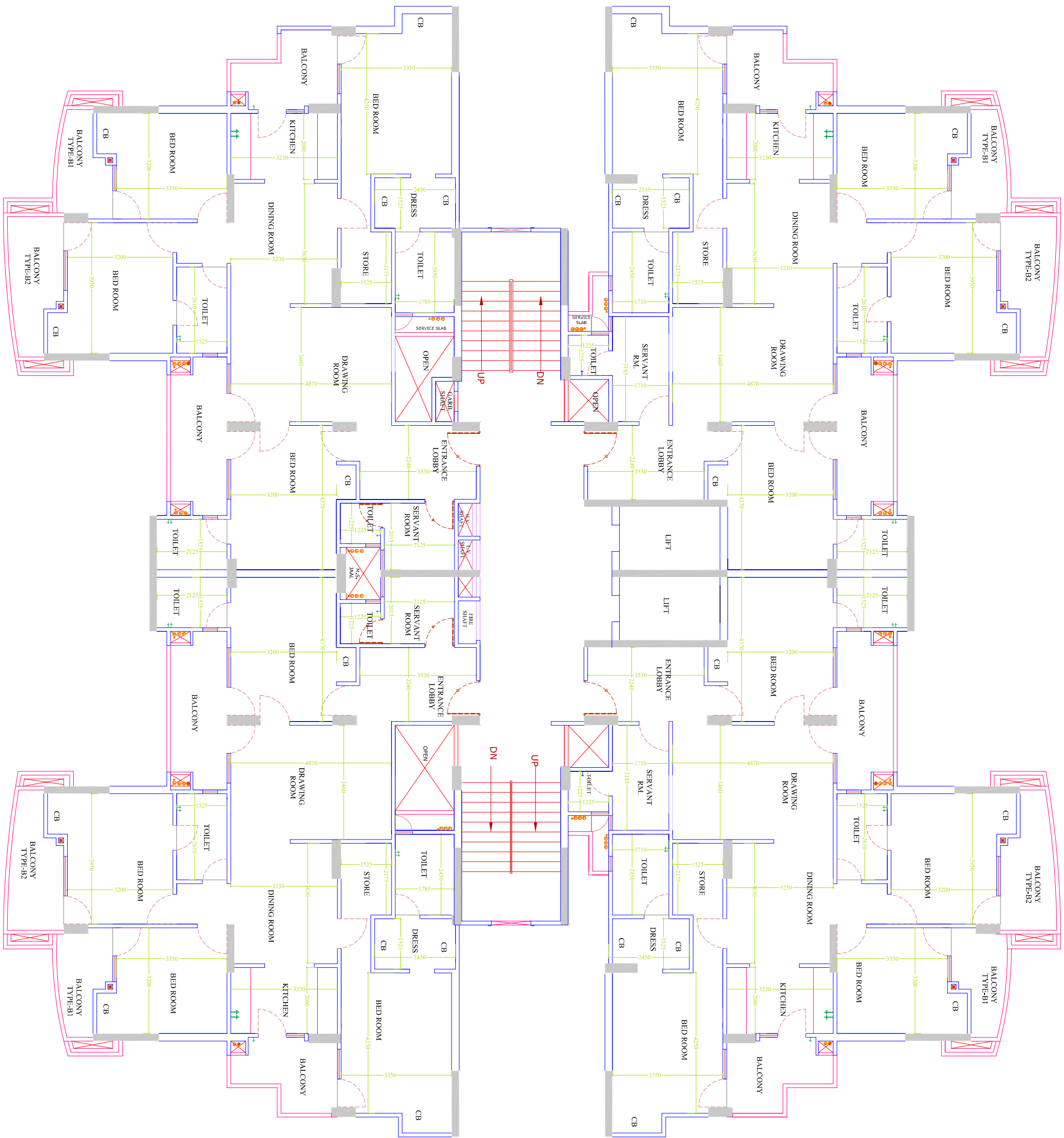
TOWER-G1 TYPICAL FLOOR PLAN
