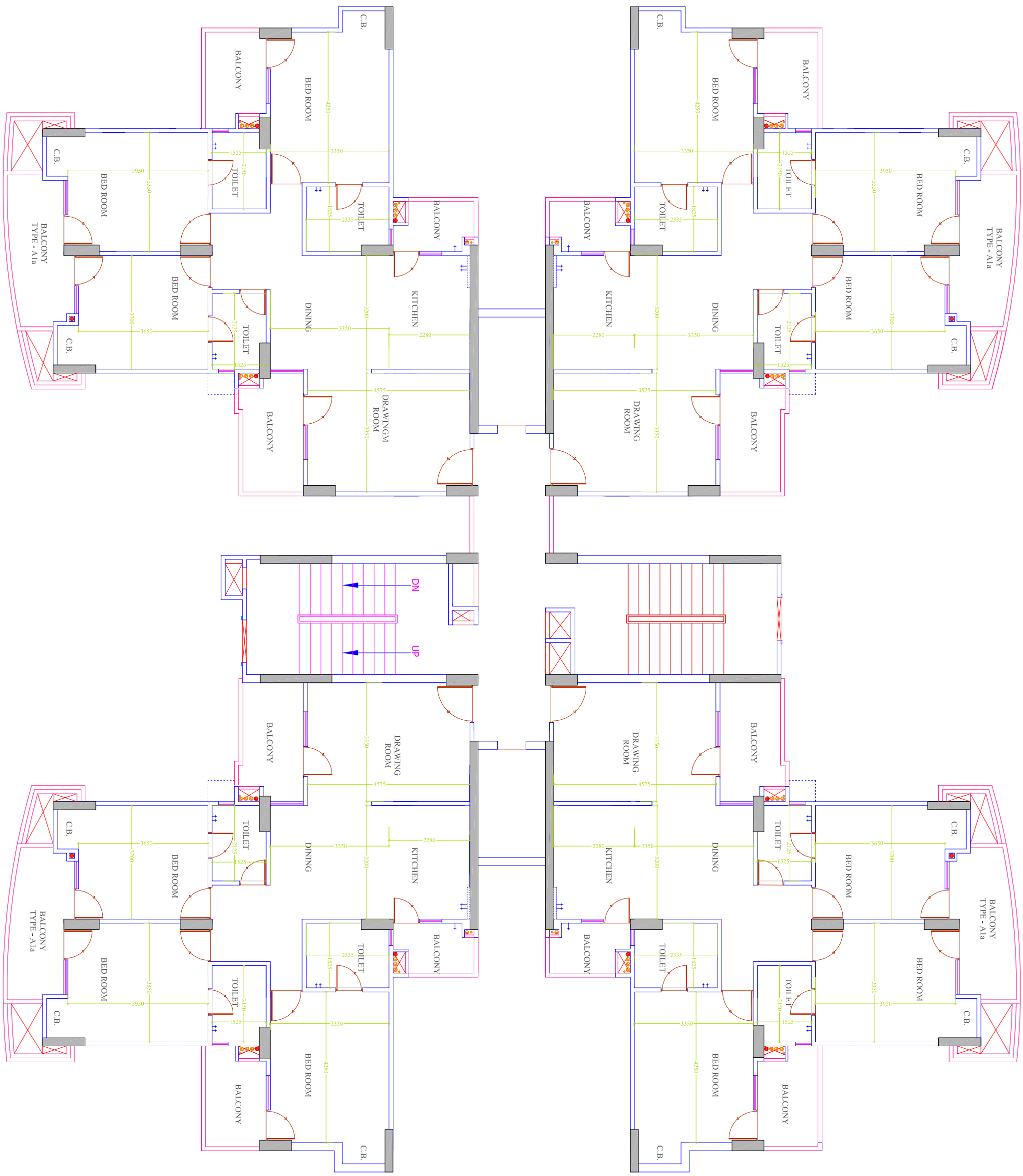
TOWER-E4 TYPICAL FLOOR PLAN
