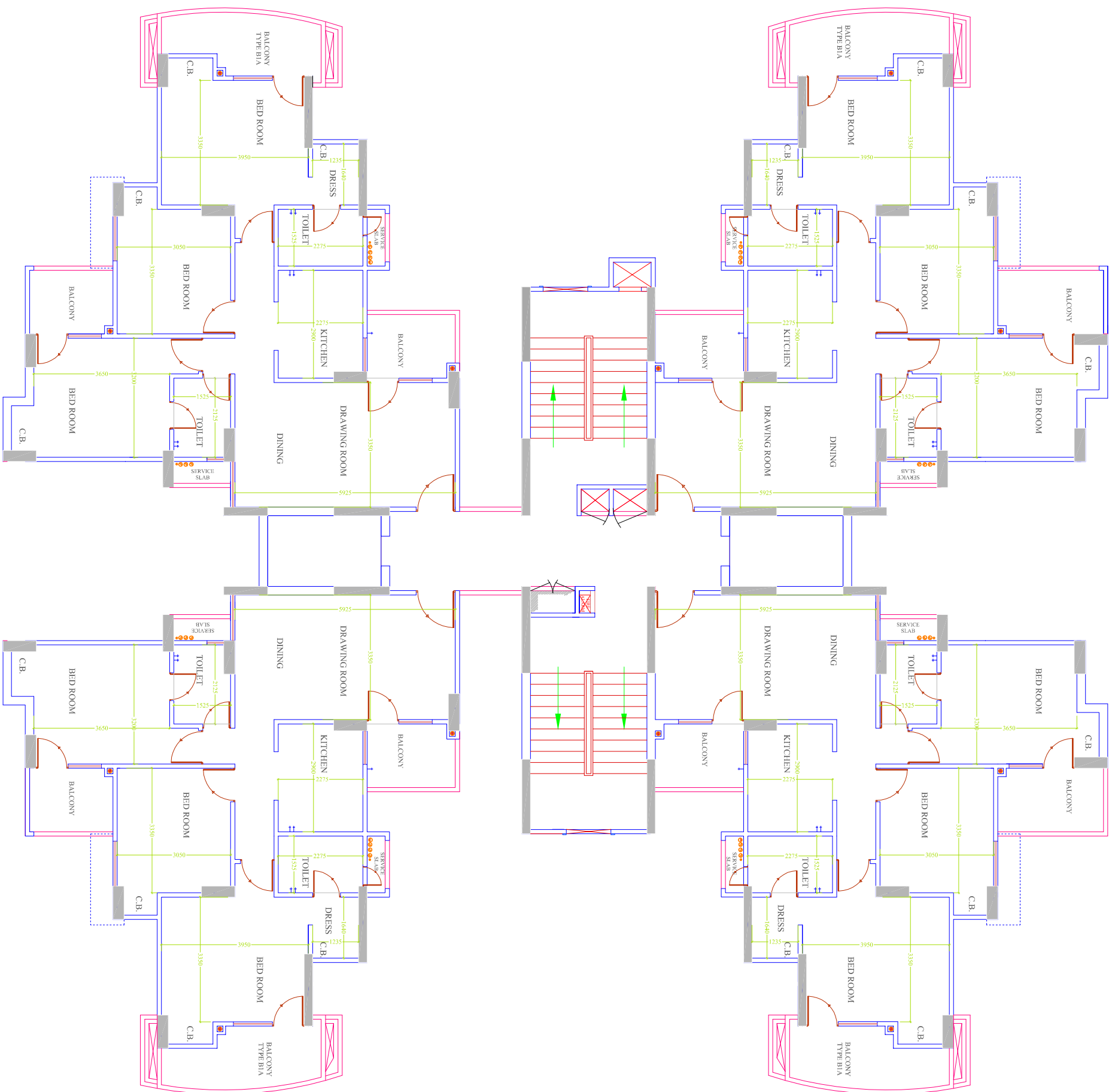
TOWER-D5 TYPICAL FLOOR PLAN
