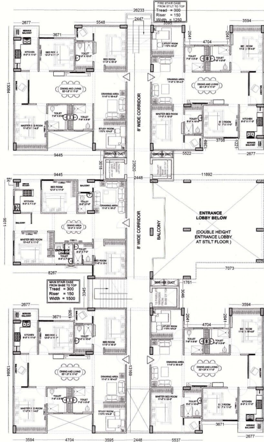
1ST FLOOR PLAN (TOWER- 3,4 &5 )
