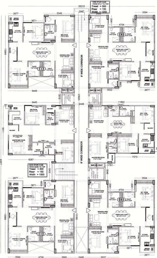
2ND TO 12 TH FLOOR PLAN (TOWER- 3,4 &5 )
