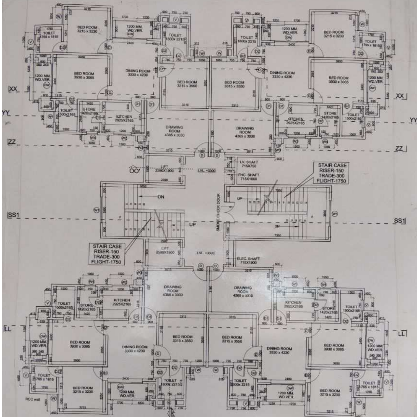
TYPICAL FLOOR PLAN-1st to 12th Floor
