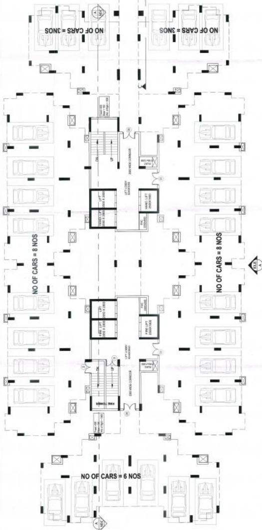
GROUND FLOOR PLAN TOWER - E - CONVENIENT SHOPPING NO. OF CARS - 28 NOS
