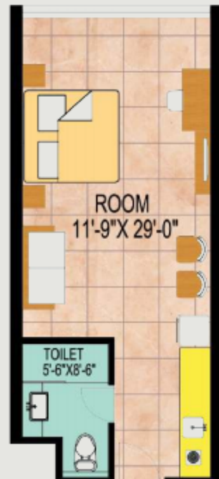
TYPE M1 9TH TO 12TH FLOOR
