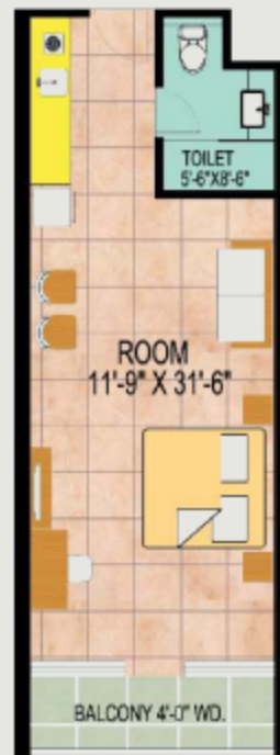
TYPE J 9TH TO 12TH FLOOR
