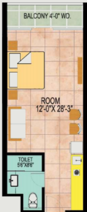
TYPE B 1 9TH TO 12TH FLOOR
