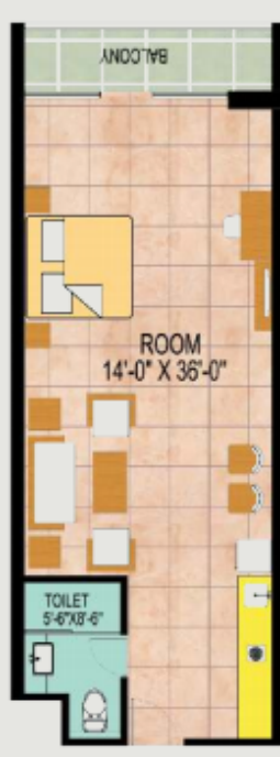
TYPE G 9TH TO 12TH FLOOR
