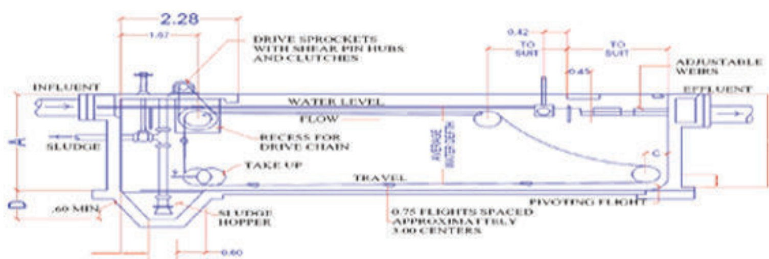
STP TANK DETAIL SCALE-N.T.S.
