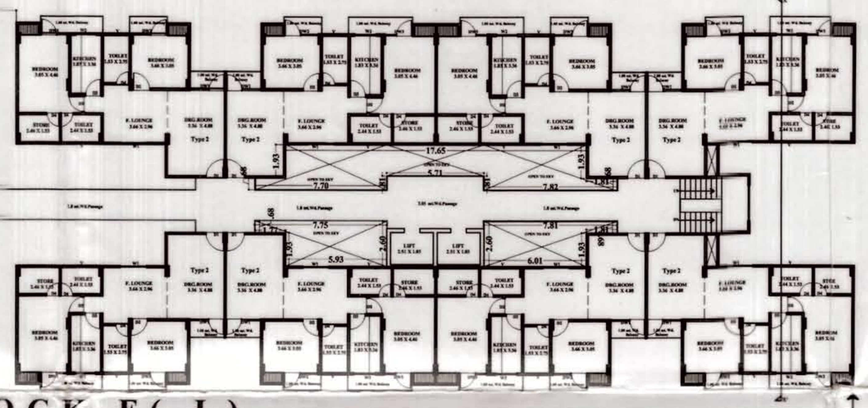
10th. FLOOR to 12th. FLOOR BLOCK F (L)
