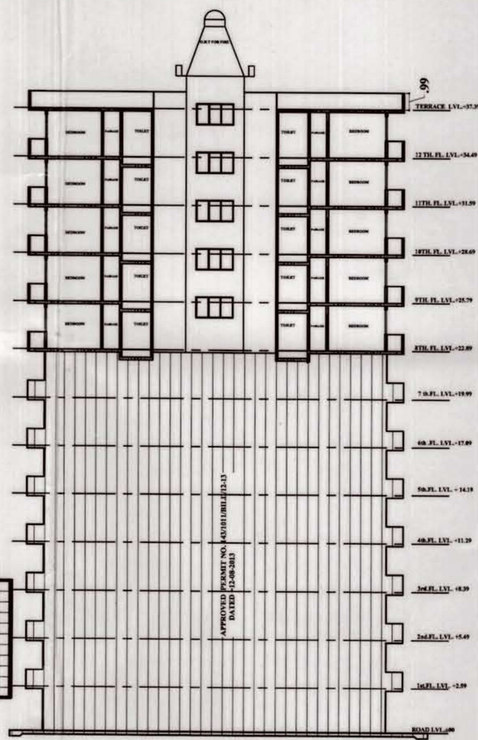
SECTION BLOCK M
