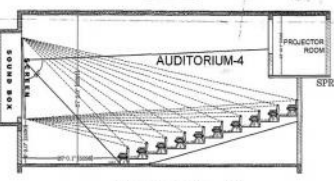
SECTION AT-AA
