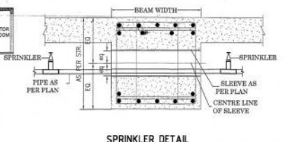
SPRINKLER DETAIL
