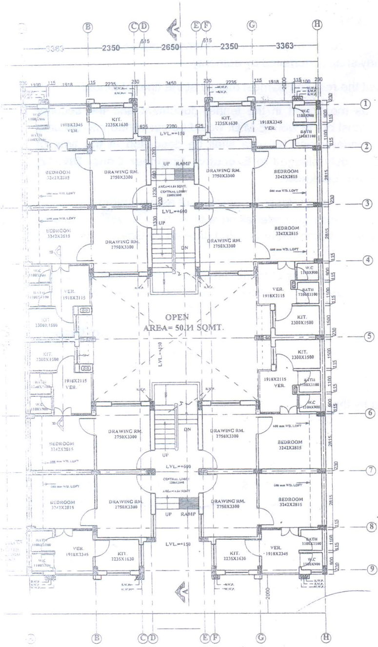
GROUND FLOOR PLAN (WORKING DRAWING)
