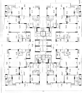
TYPICAL FLOOR PLAN (1ST TO 15TH FLOOR)
