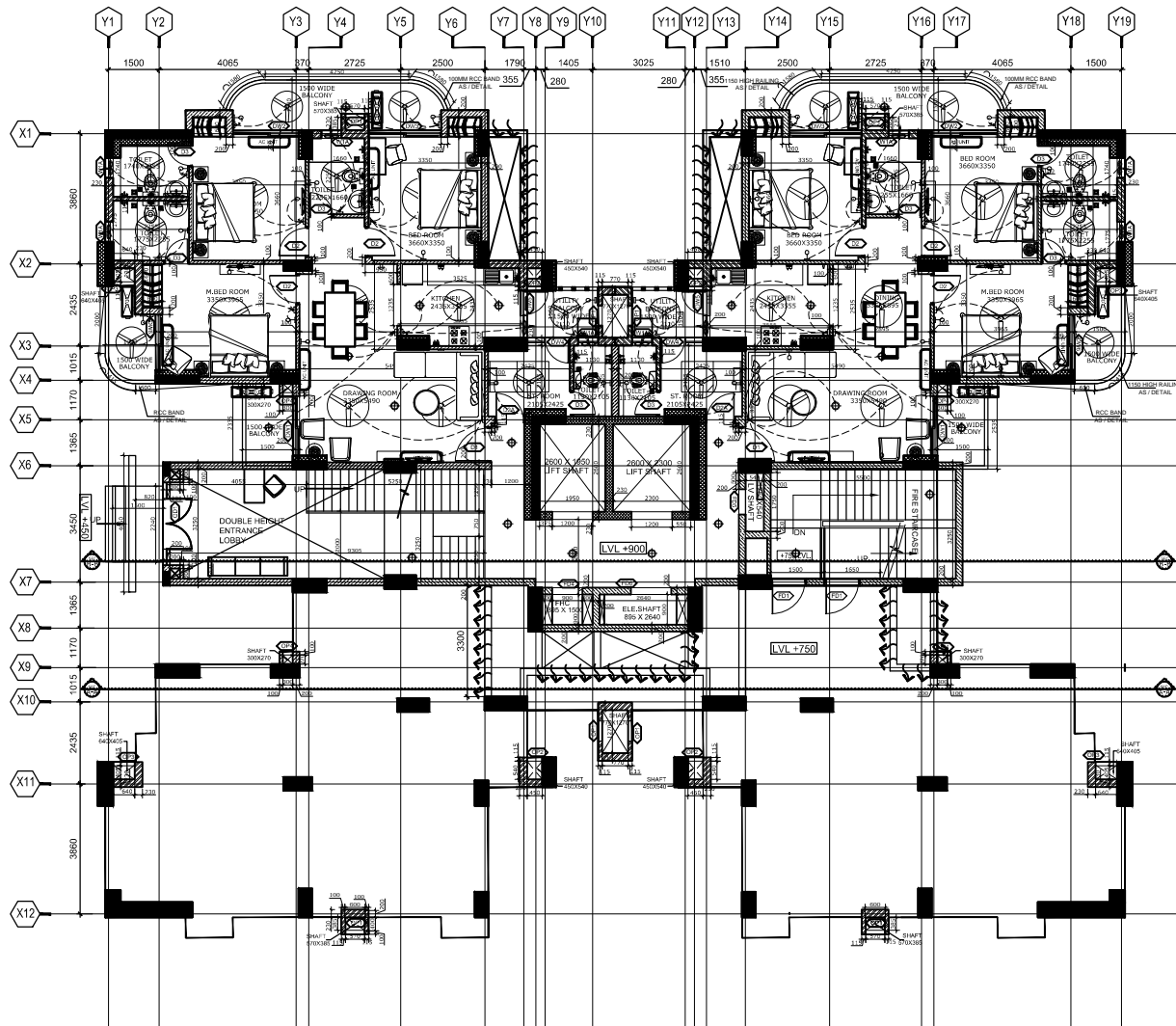
STILT/GROUND FLOOR LVL
