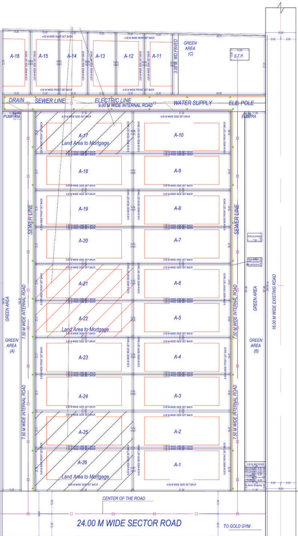
SERVICE PLAN SCALE 1:100
