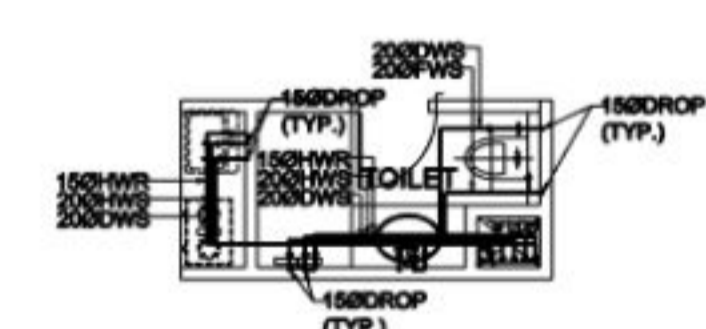
TOILET DETAIL DRAINAGE LAYOUT & WATER SUPPLY LAYOUT
