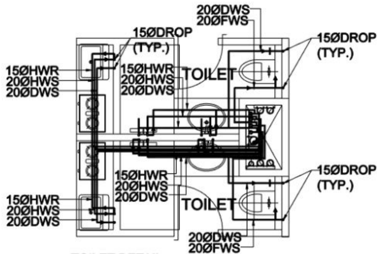
TOILET DETAIL DRINAGE LAYOUT & WATER SUPPLY LAYOUT
