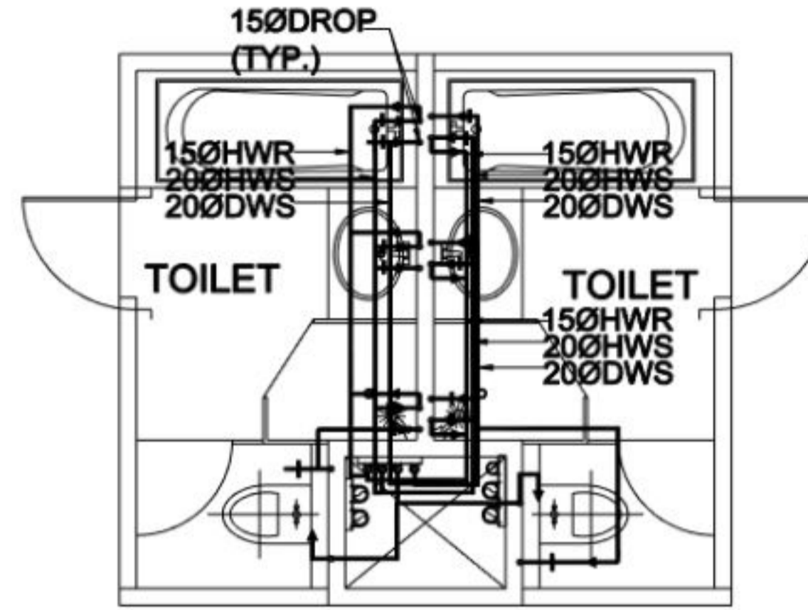
TOILET DETAIL DRINAGE LAYOUT & WATER SUPPLY LAYOUT
