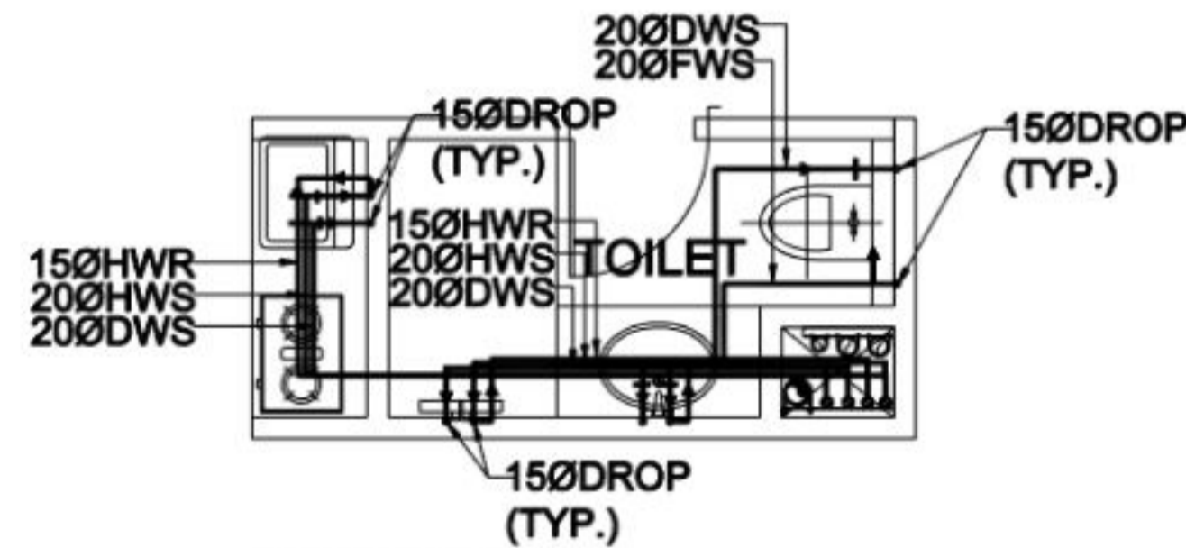
TOILET DETAIL DRINAGE LAYOUT & WATER SUPPLY LAYOUT
