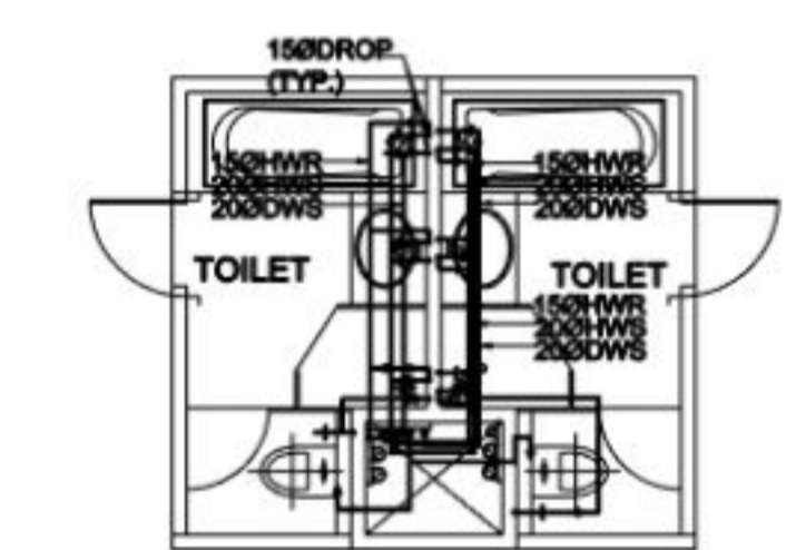
TOILET DETAIL DRAINAGE LAYOUT & WATER SUPPLY LAYOUT
