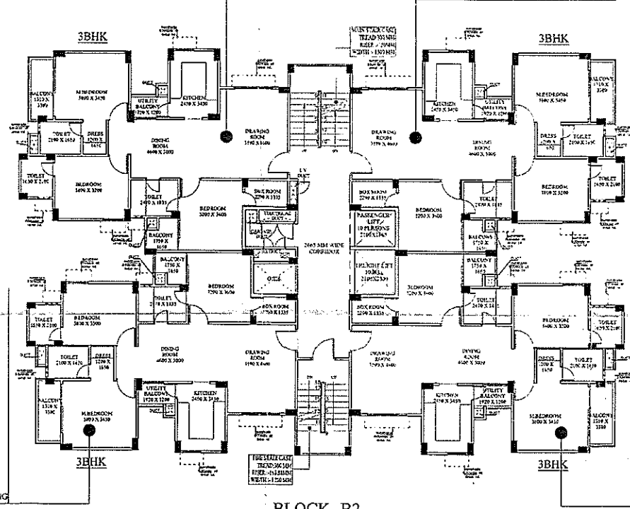
BLOCK - B2 TYPICAL FLOOR PLAN
