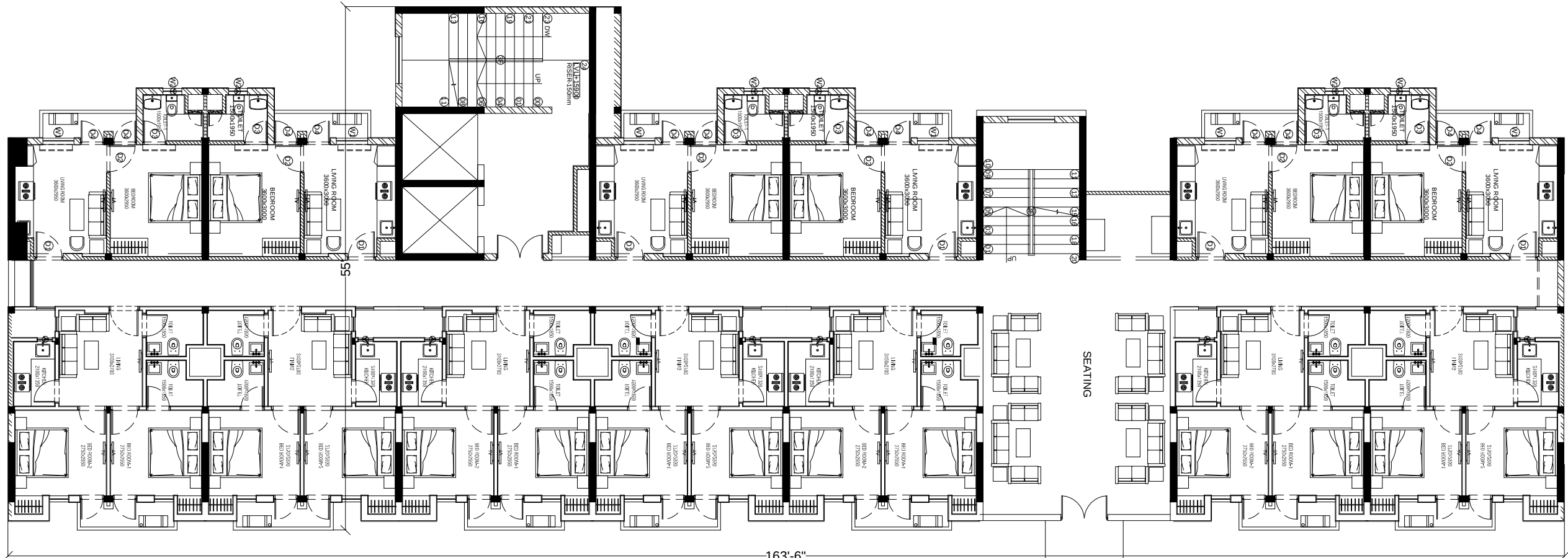
SECOND FLOOR
