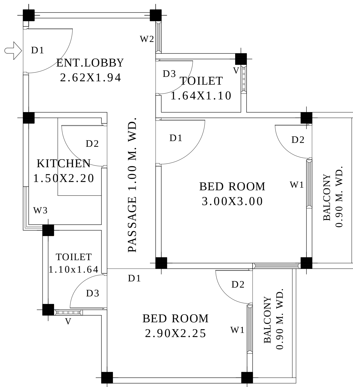
LIG HOUSES UNit Plan
