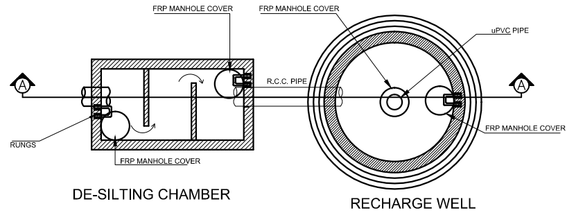
PLAN OF PHASE-1 DE - SELTING CHAMBER & RECHARGE WELL
