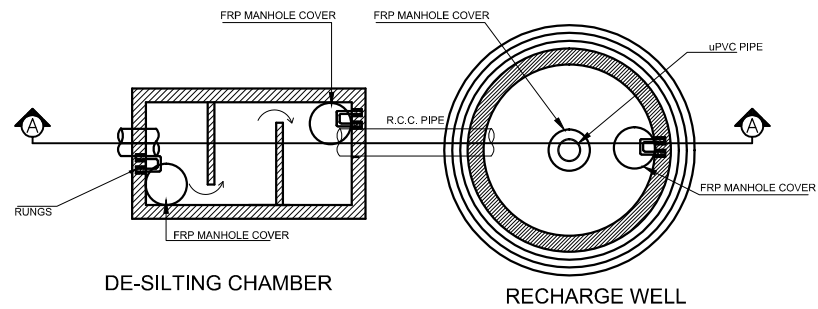
PLAN OF PHASE-2 DE - SELTING CHAMBER & RECHARGE WELL
