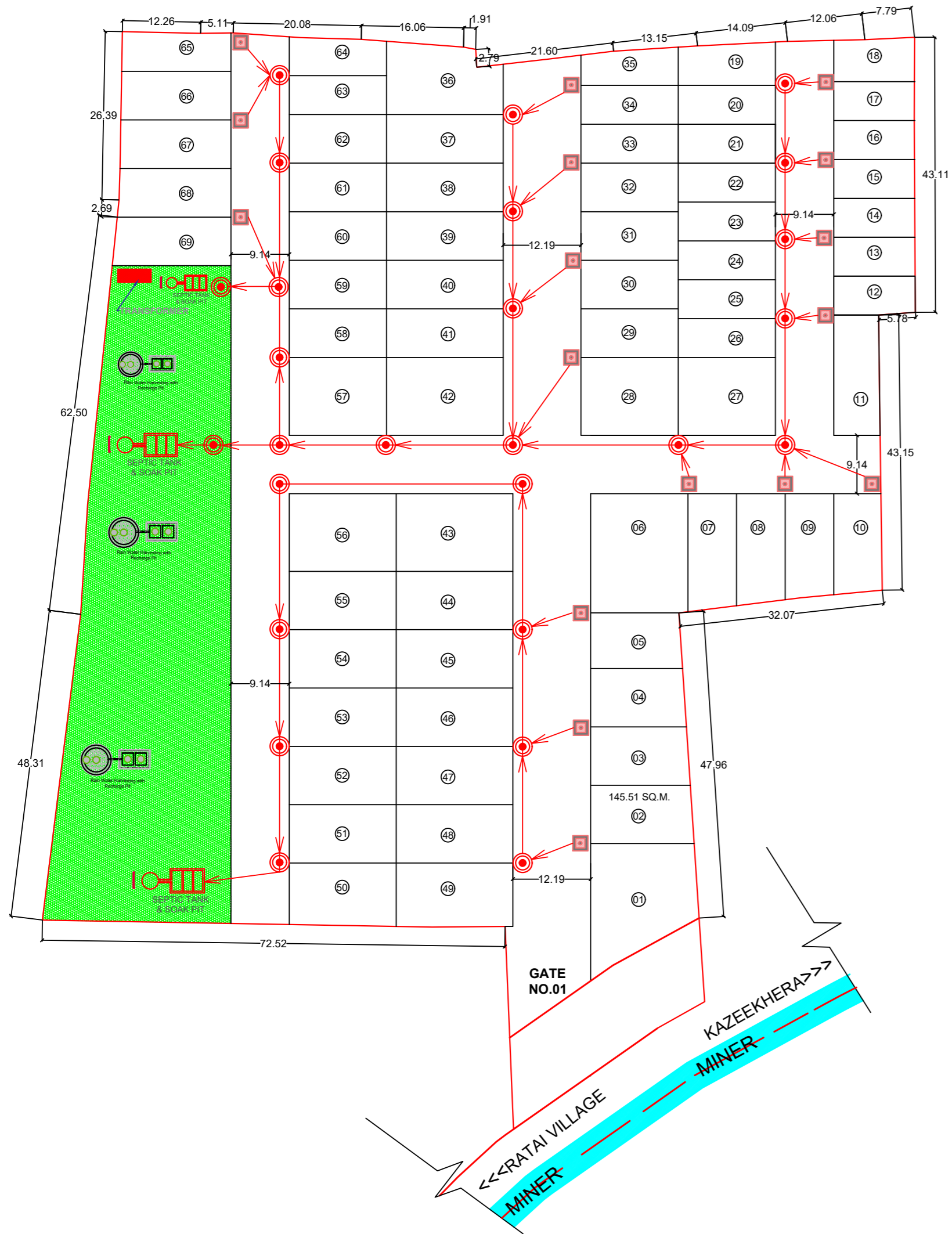
SEWER LAYOUT PLAN SCAL 1:500
