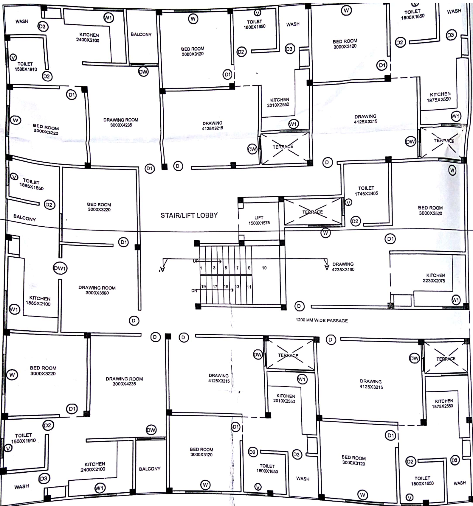
TYPICAL FLOOR PLAN (STILT+1, TO ,STILT+4) SCALE 1:100
