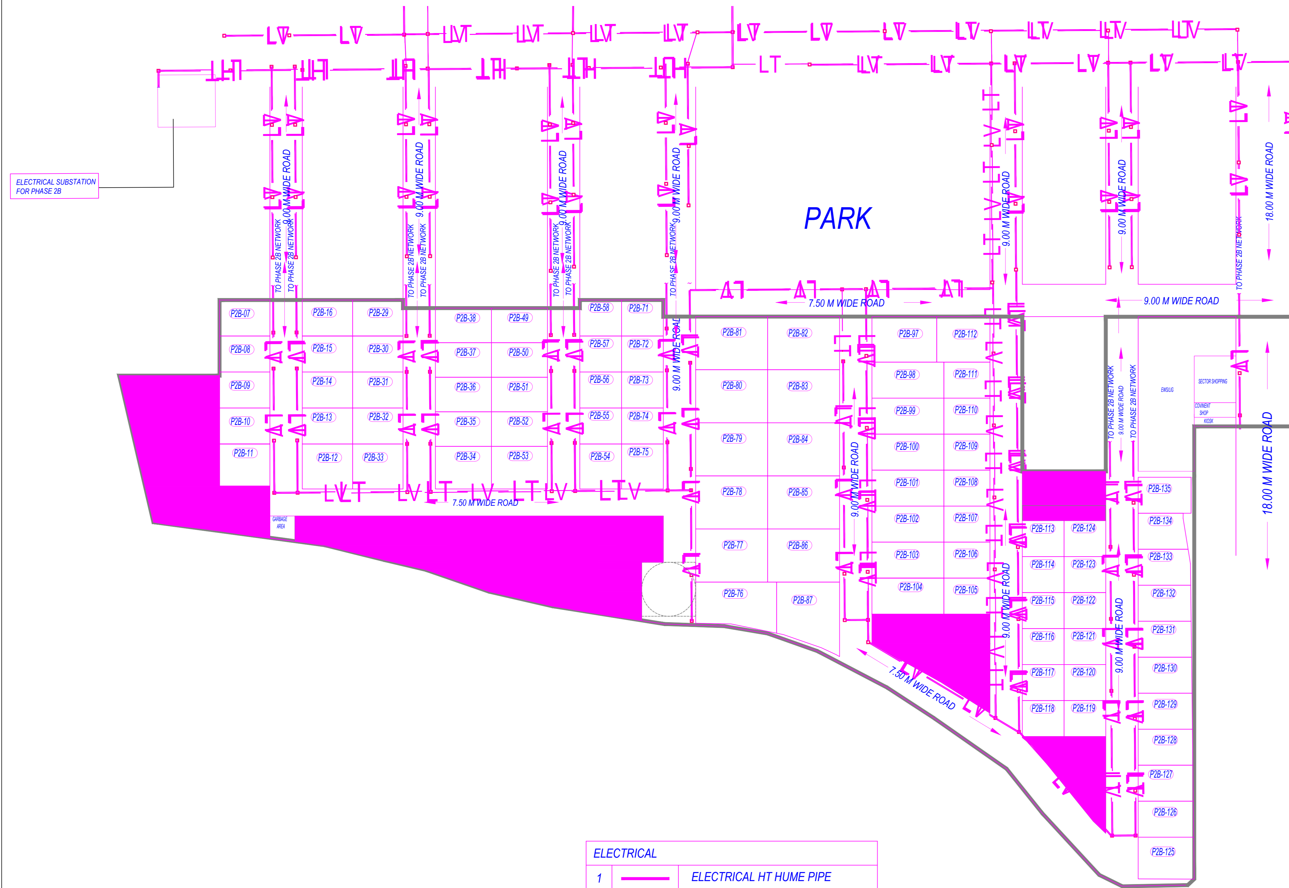
ELECTRICITY PLAN
