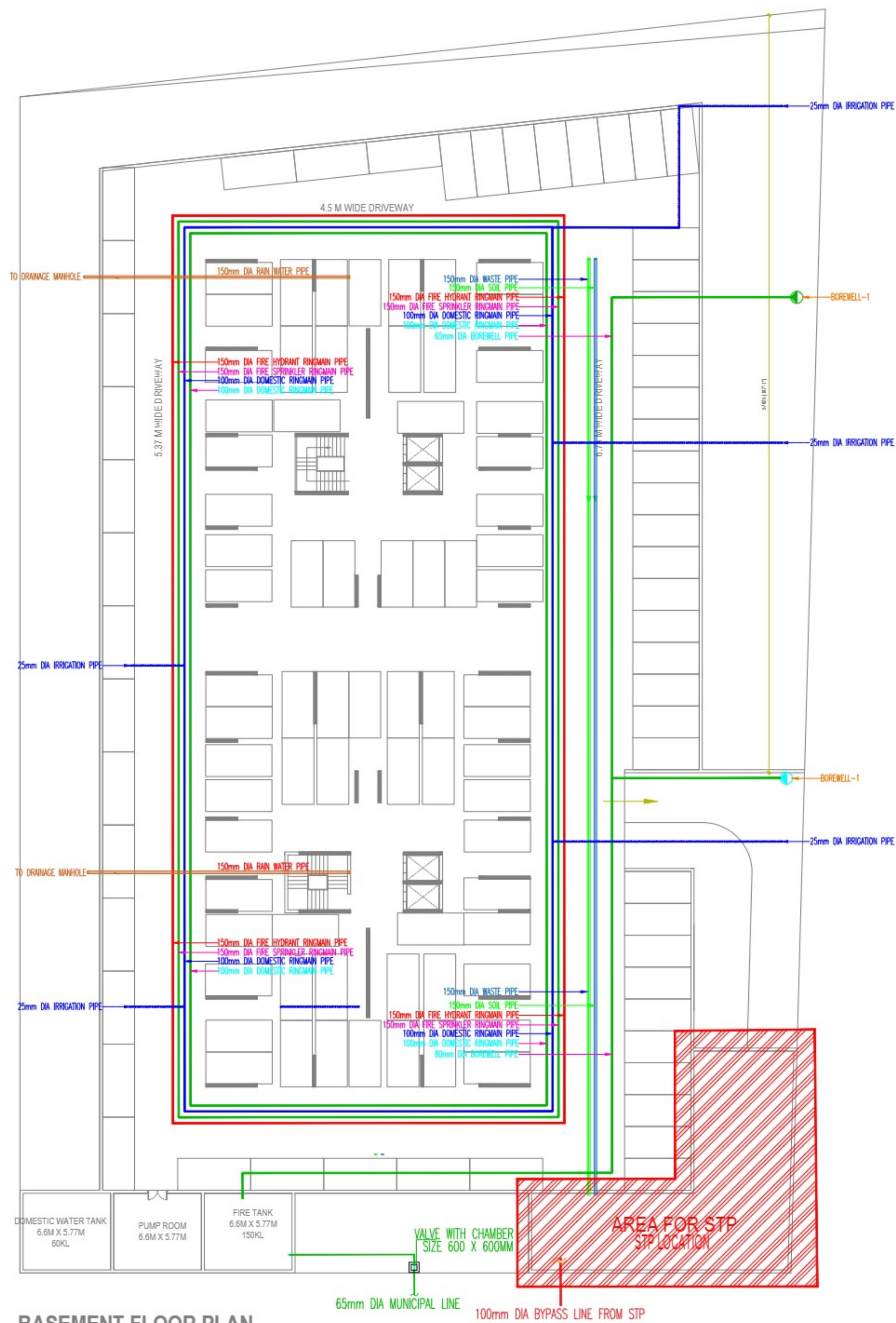
BASEMENT FLOOR PLAN
