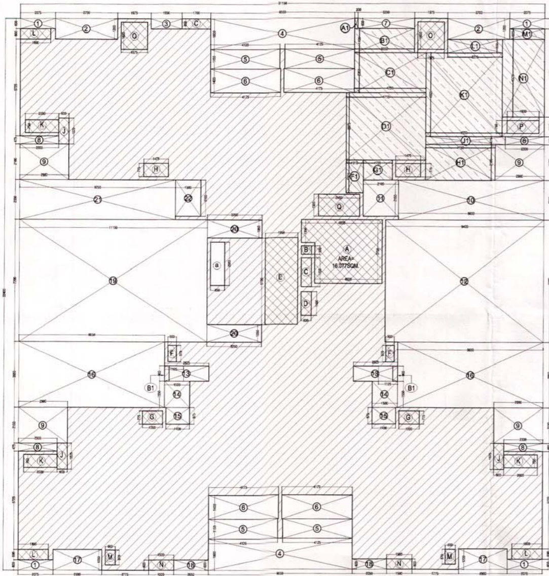
STILT/GROUND FLOOR AREA DETAIL PLAN
