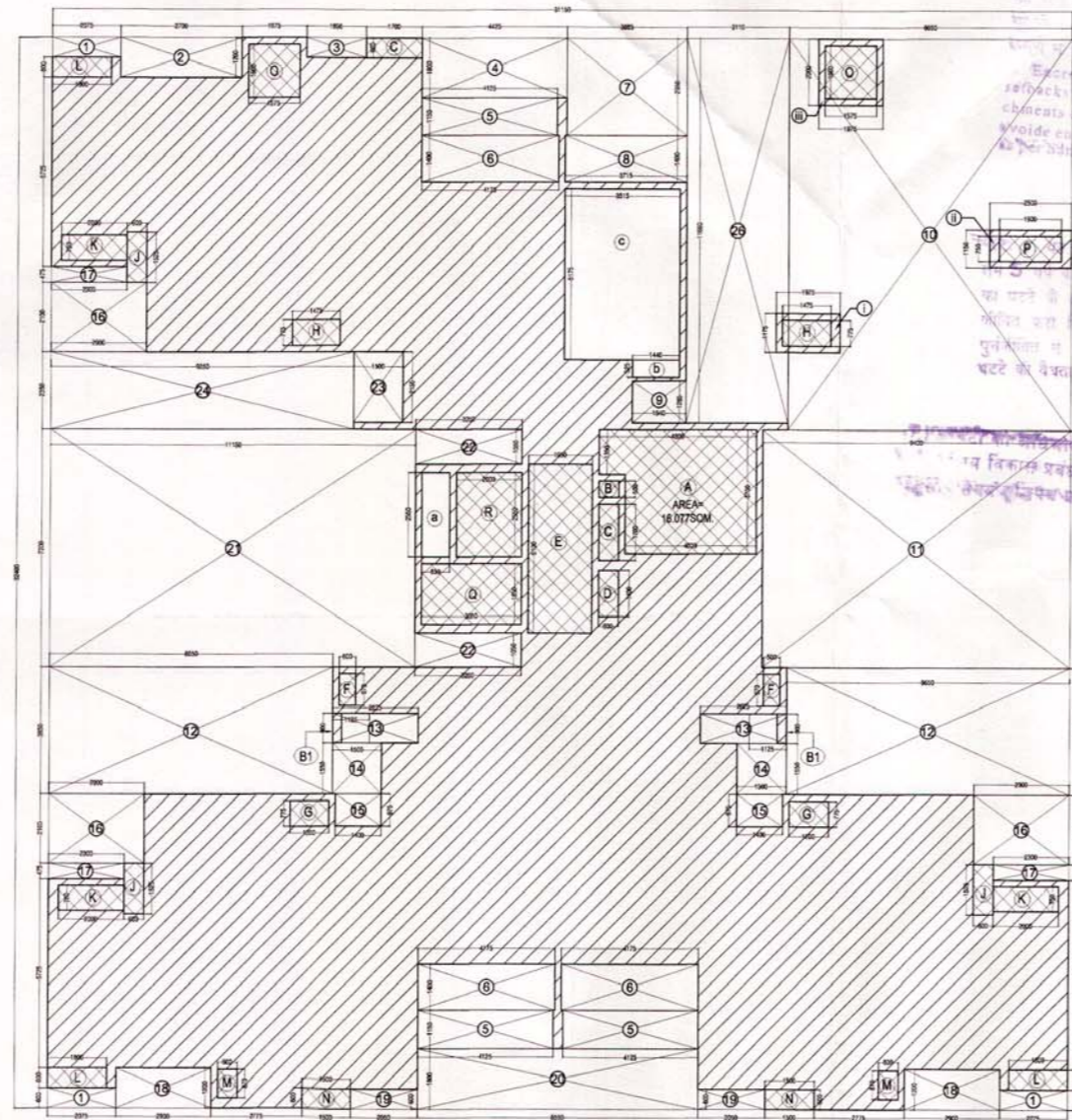
FIRST FLOOR AREA DETAIL PLAN
