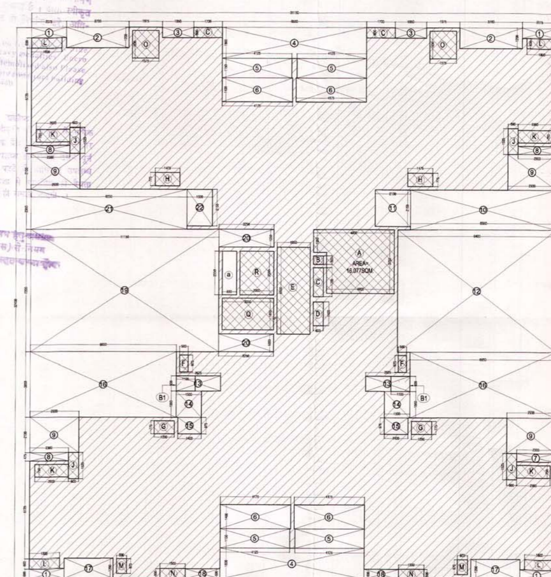
TYPICAL FLOOR AREA DETAIL PLAN
