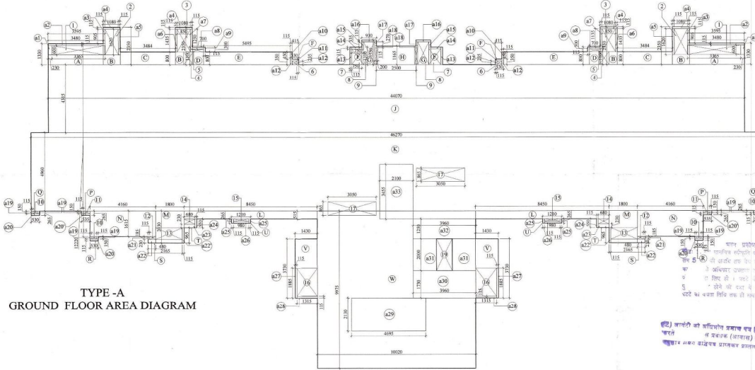
TYPE-A GROUND FLOOR PLAN
