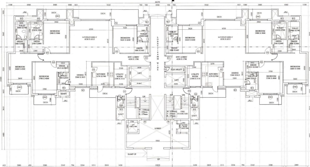
TYPE-A GROUND FLOOR PLAN
