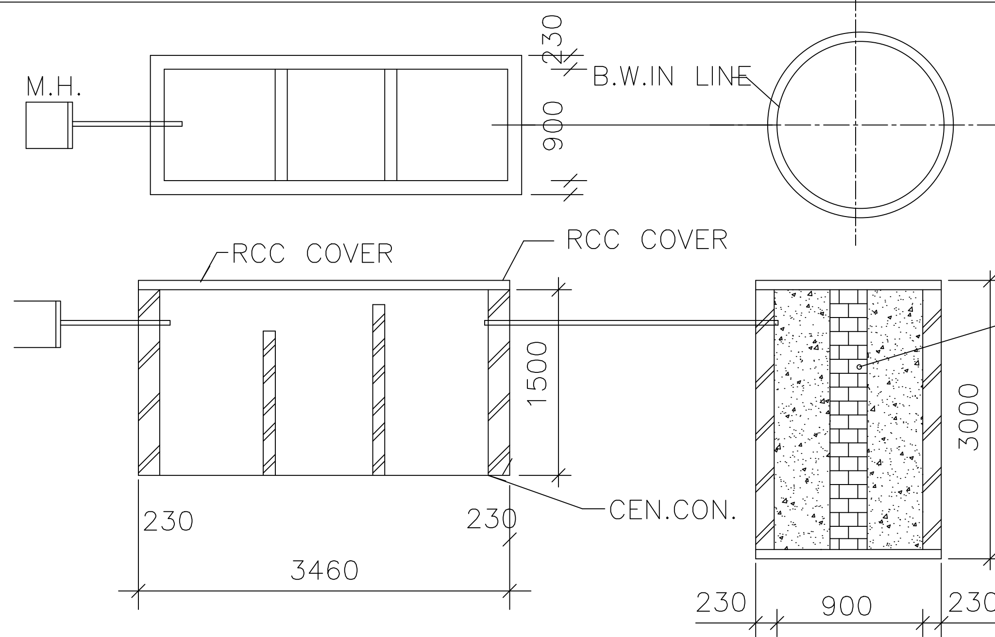
SOLID AND LIQUID WASTE TREATMENT PLANT
