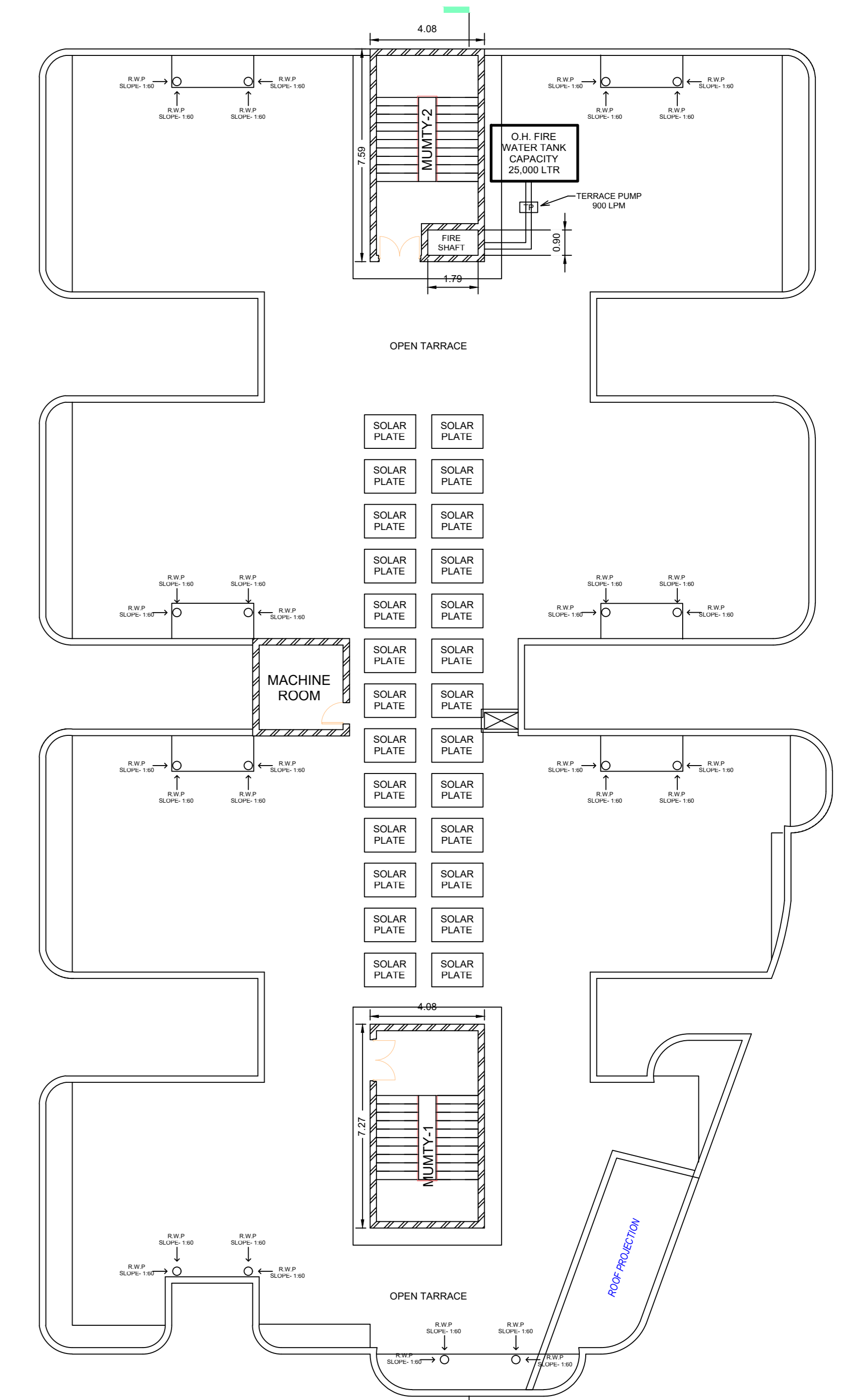
SERVICE PLAN SCALE 1:150
