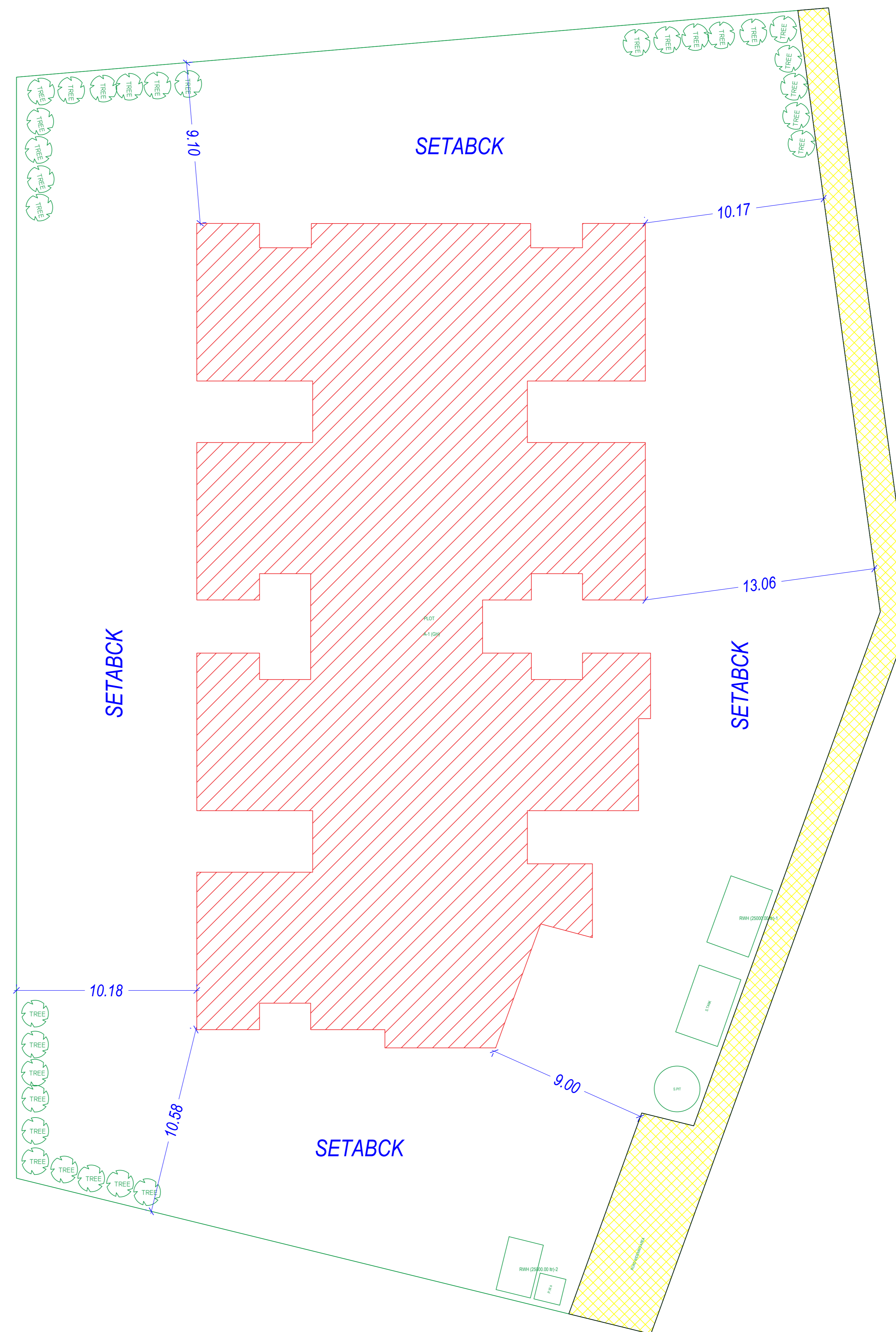
LANDSCAPE PLAN SCALE 1:150
