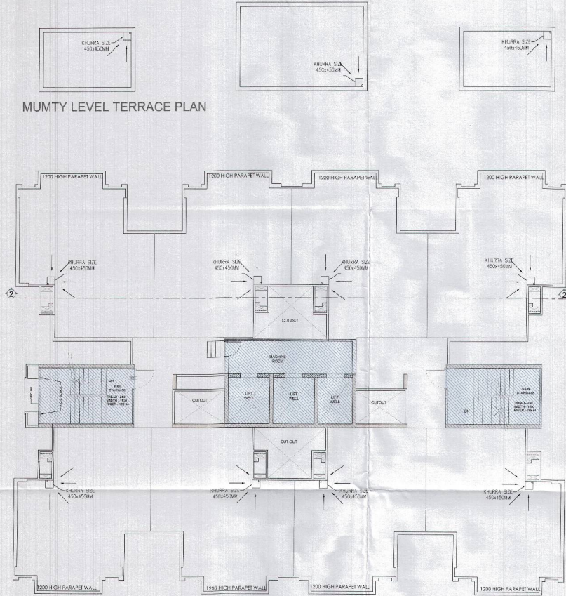
TERRACE PLAN
