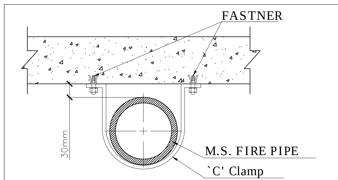
TYPICAL PIPE CLAMP DETAIL
