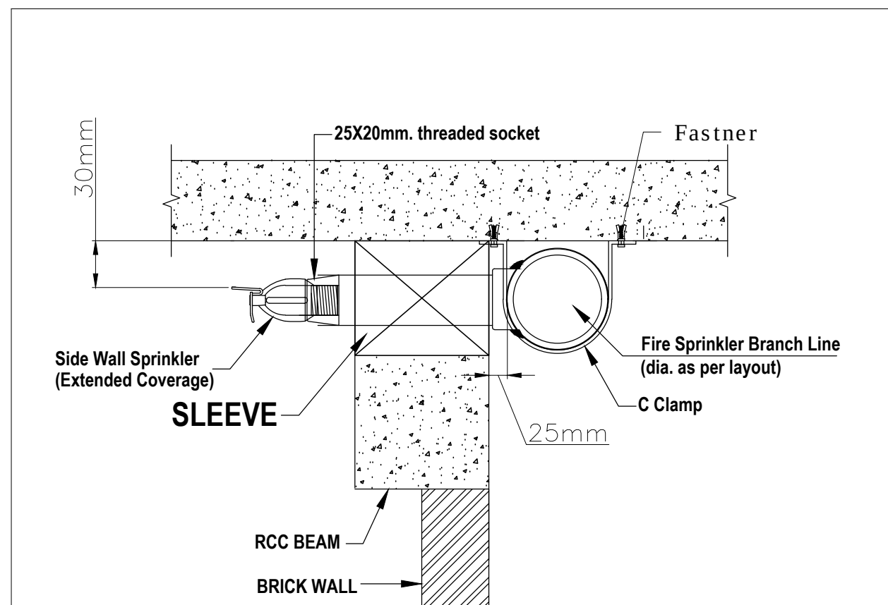
ELEVATION -LONG THROW SPRINKLER
