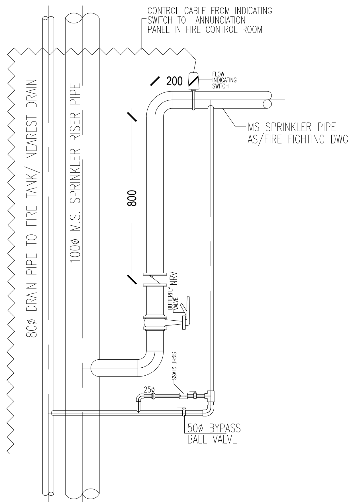
INSPECTION TEST ASSEMBLY
