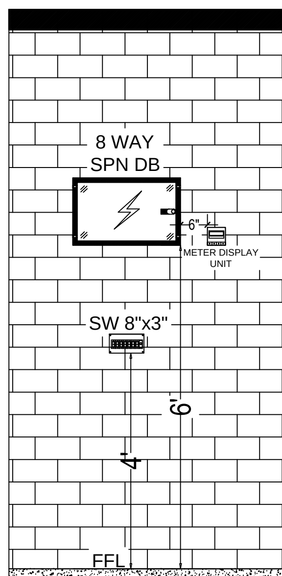
MCB DB & SWITCH BOARD POSITION ON WALL FOR SHOP HAVING 1 FAN
