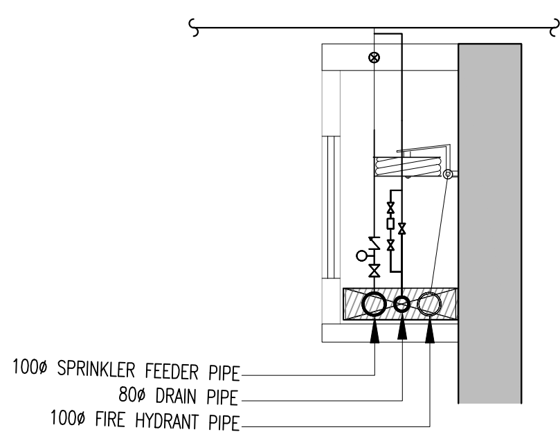
TYPICAL FIRE SHAFT-2
