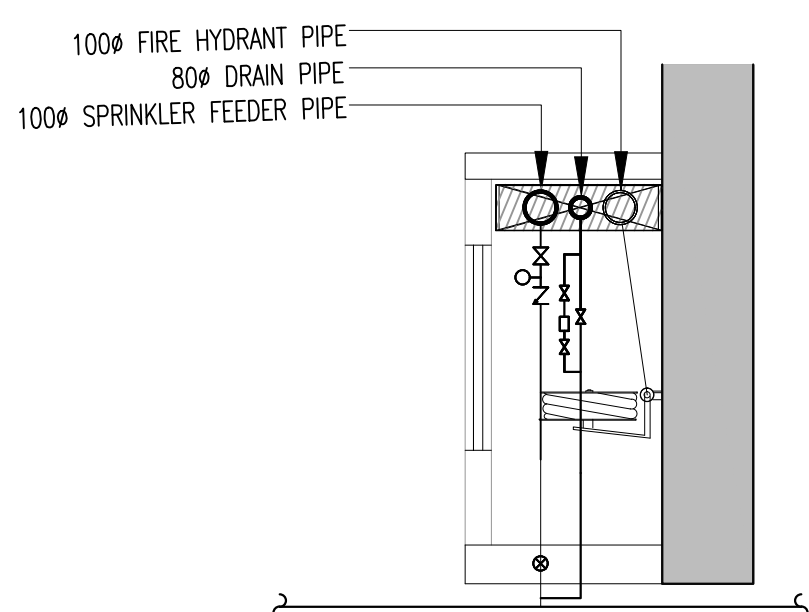
TYPICAL FIRE SHAFT-2
