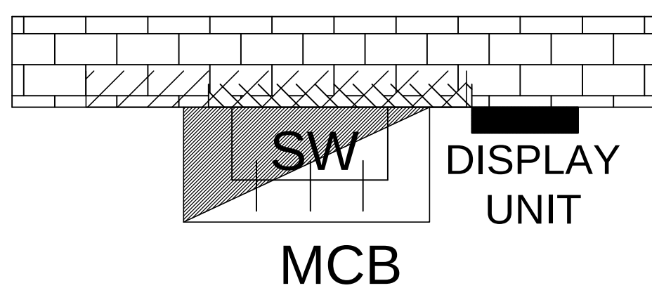
MCB DB, SWITCH BOARD & DISPLAY UNIT POSITION ON WALL FOR EACH SHOP (TOP VIEW)
