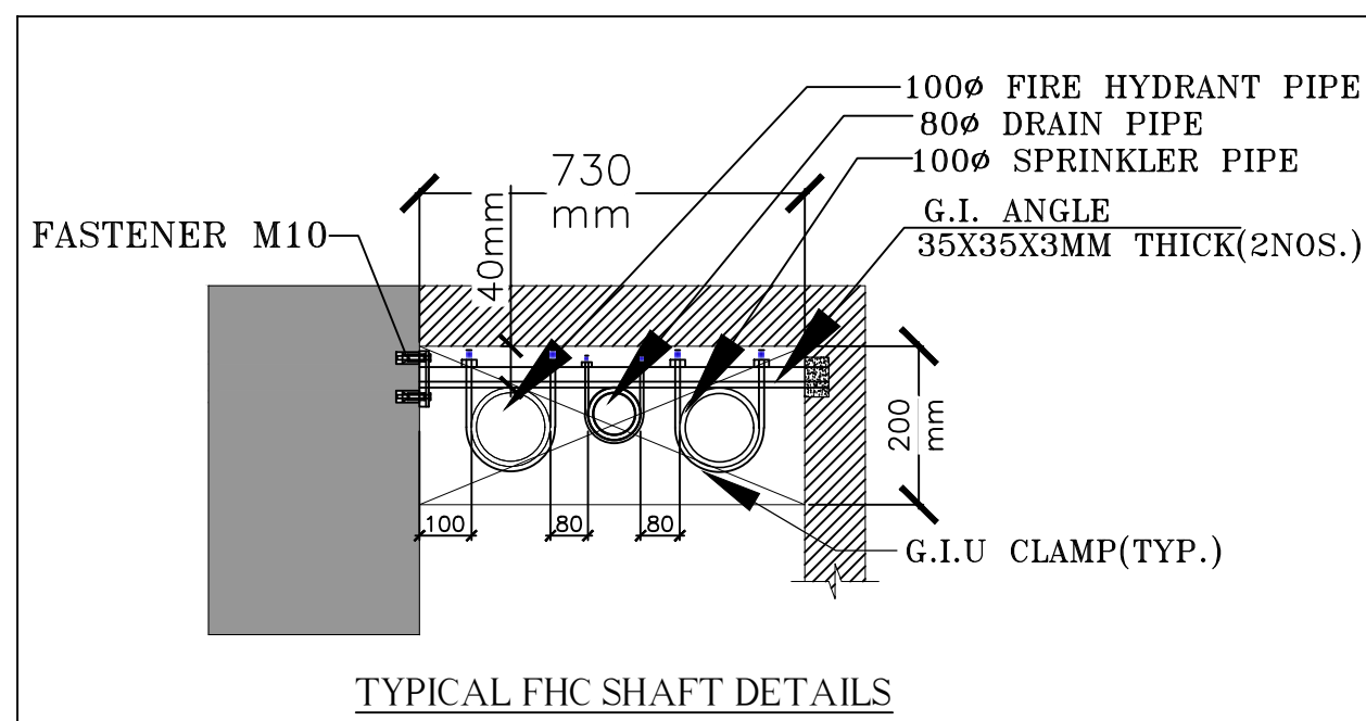
TYPICAL FHC SHAFT DETAILS
