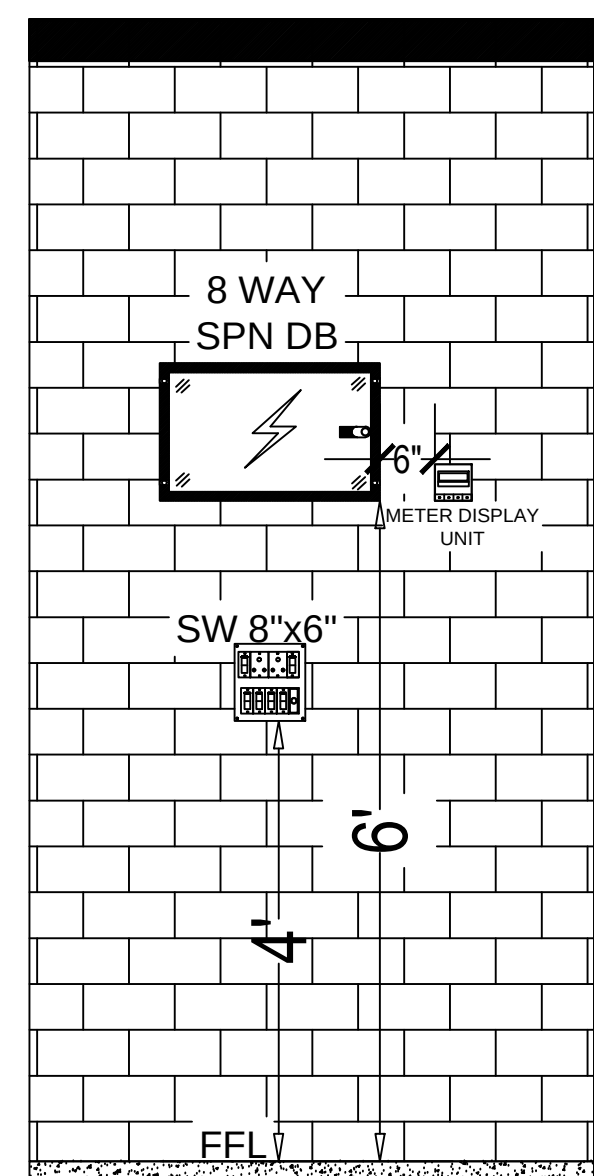
MCB DB & SWITCH BOARD POSITION ON WALL FOR SHOP HAVING 2 FANS OR MORE
