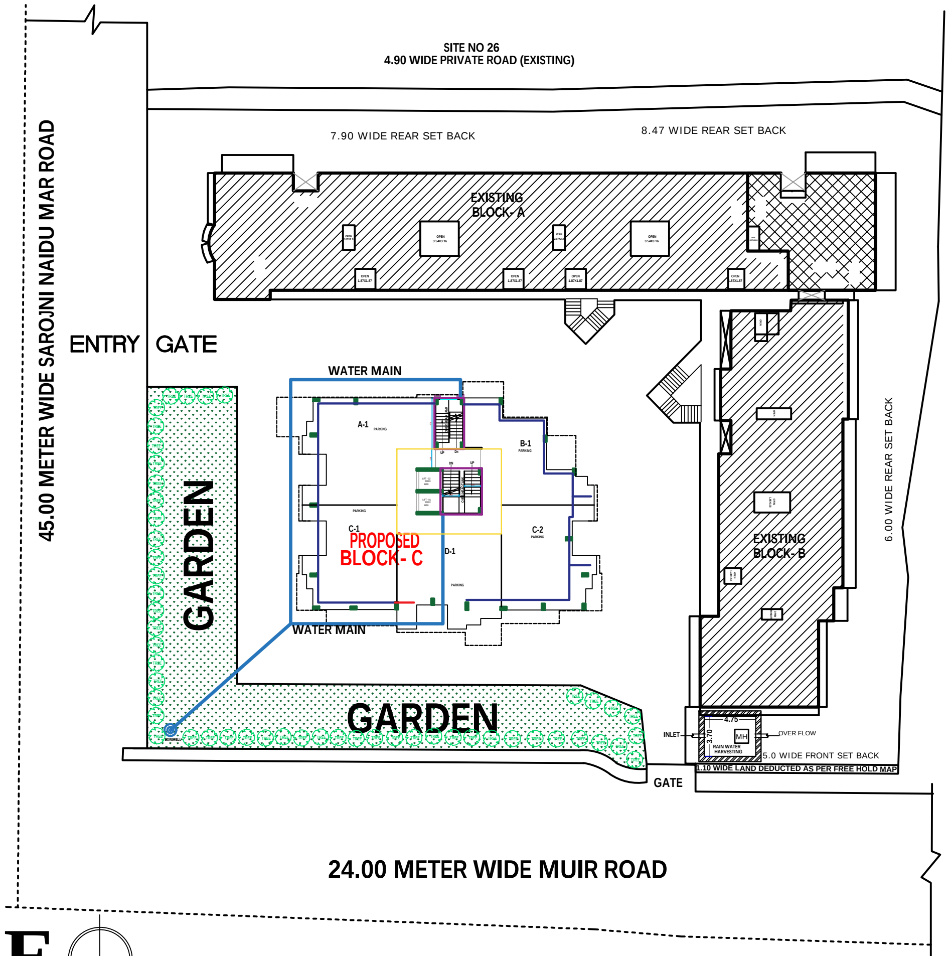
WATER SUPPLY PLAN SAIDHAM SONA APARTMENT
