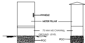
METER PILLAR DETAIL
