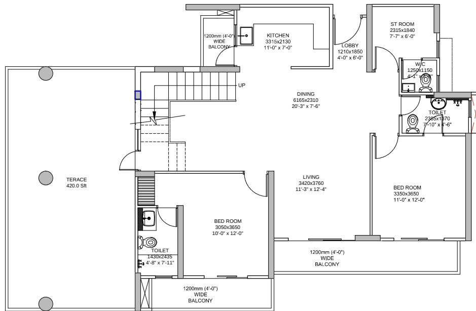
LOWER LVL
