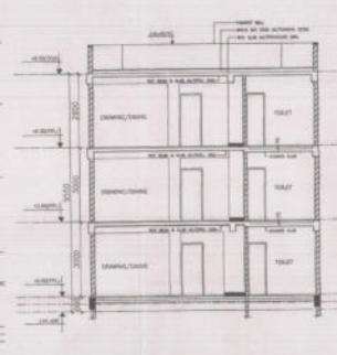
SECTION BB SCALE 1:100
