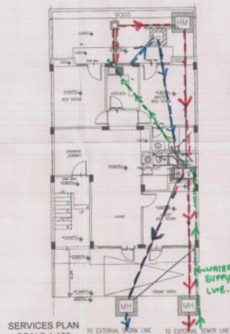
SERVICES PLAN SCALE 1:100 (PLUMBING LAYOUT)
