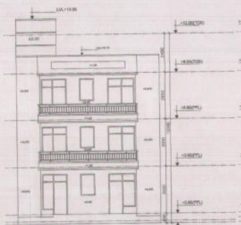
REAR ELEVATION SCALE 1:100
