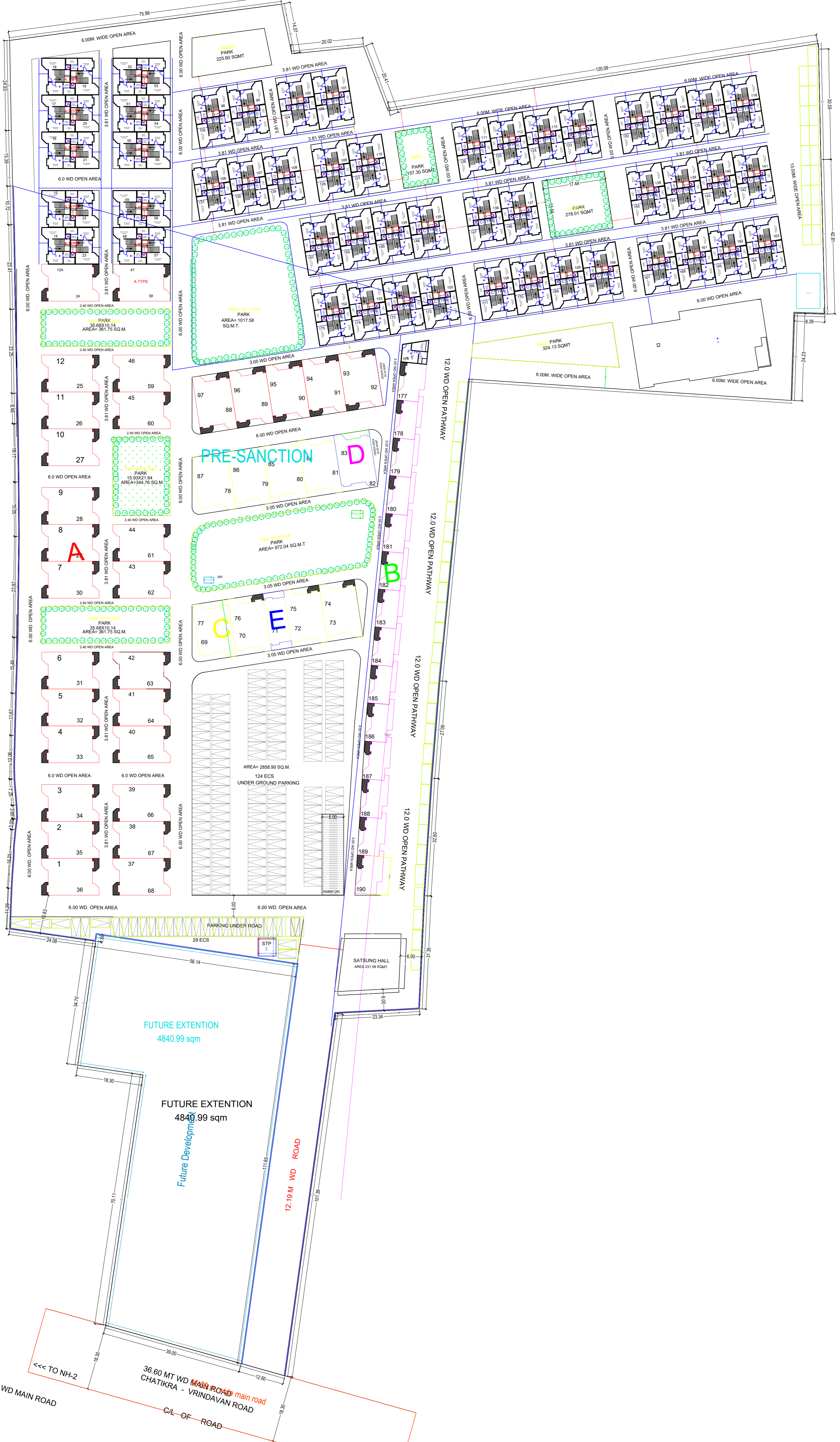
SITE PLAN
