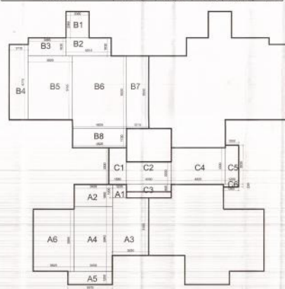
TYPICAL FLOOR(2ND TO 9TH)
