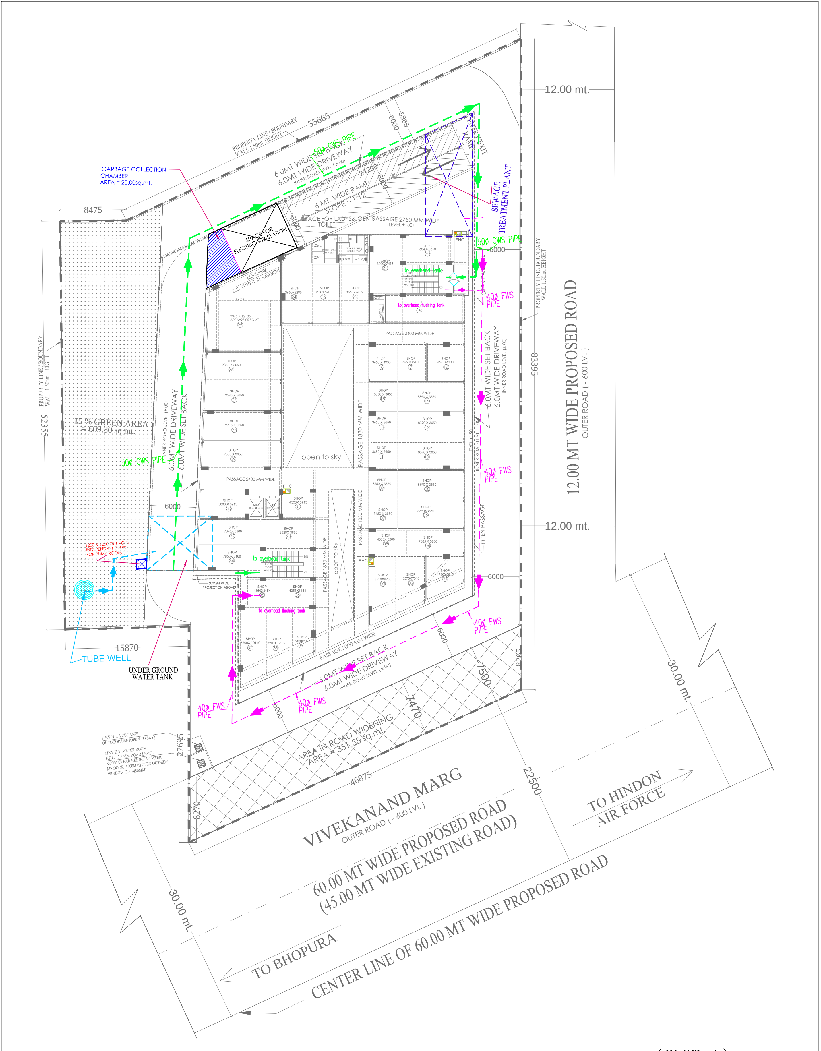
( PLOT - A ) 5.0 - INFRASTRUCTURE & SERVICES WATER SUPPLY PLAN
