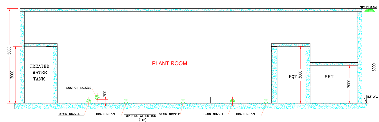
SECTION B-B
