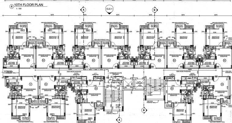
5 11TH & 12TH FLOOR PLAN 1:100
