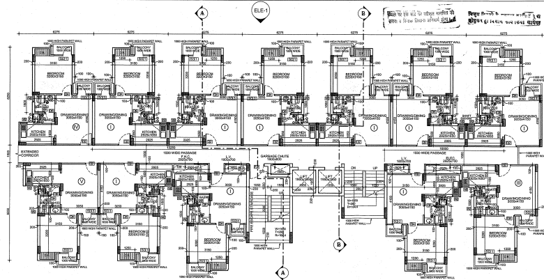
1 1ST FLOOR PLAN 1:100
