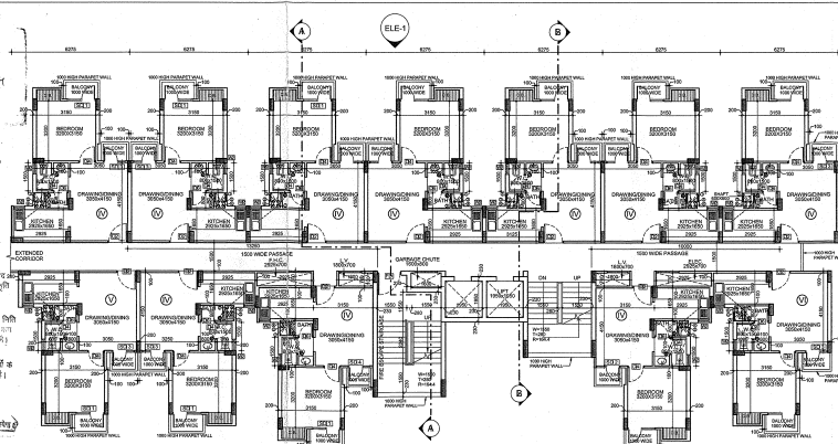
4 10TH FLOOR PLAN 1:100
