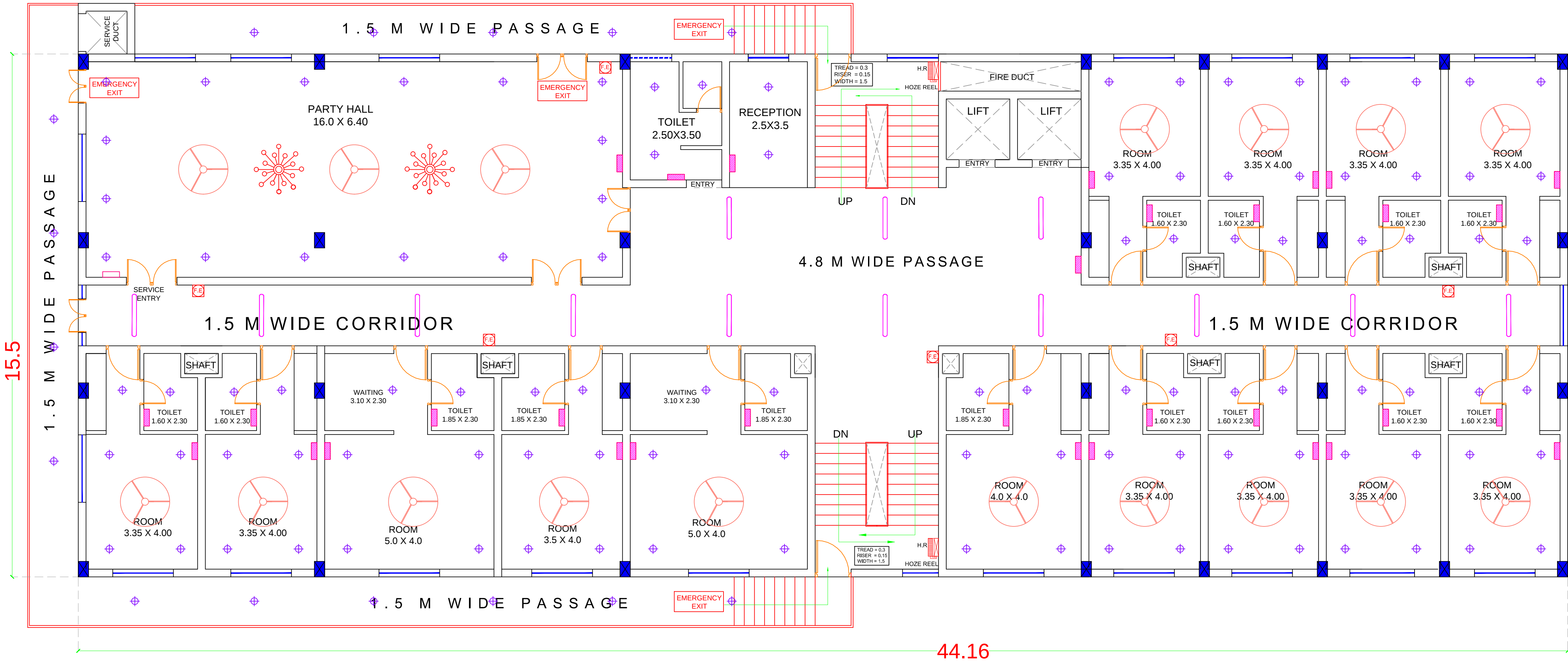
FOURTH & FIFTH FLOOR PLAN
