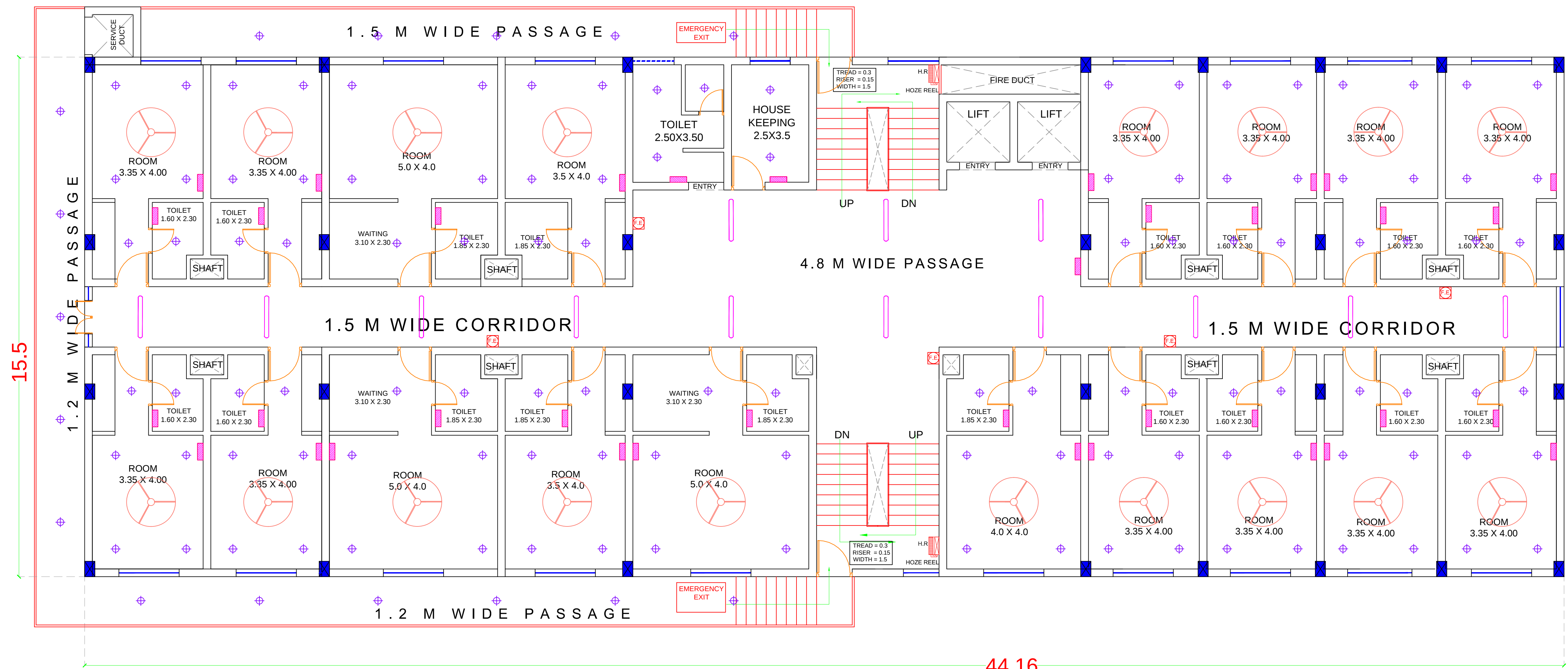
SIXTH FLOOR PLAN
