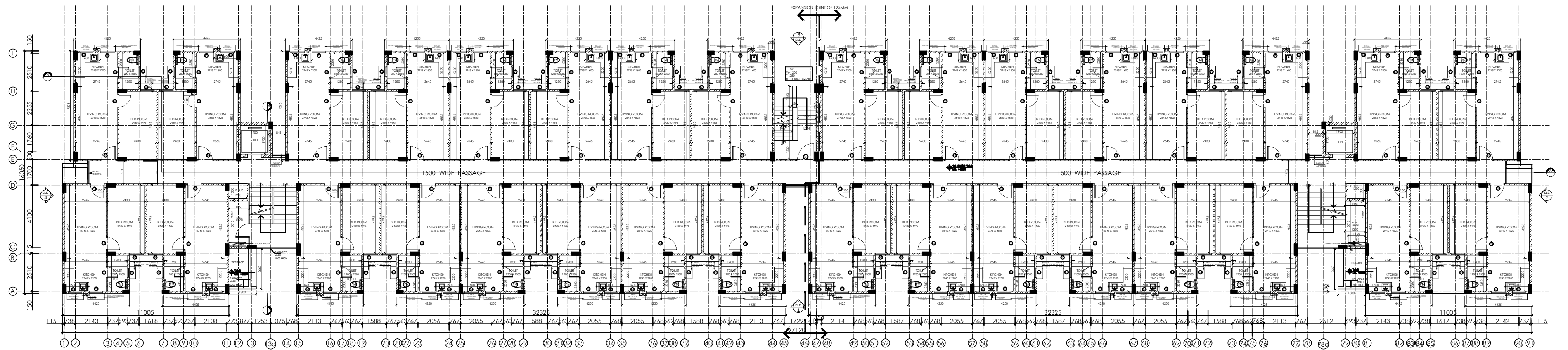
BLOCK - LIG-02, TYPICAL FLOOR PLAN
