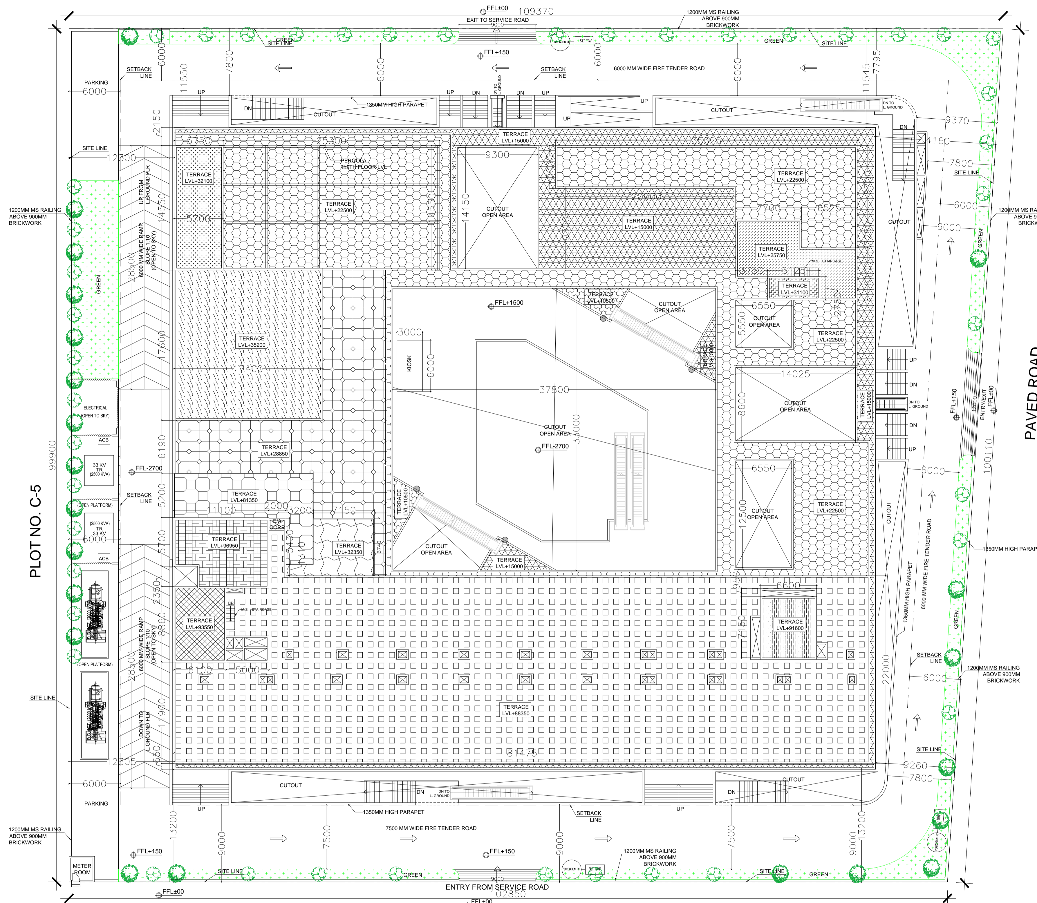
SITE PLAN
