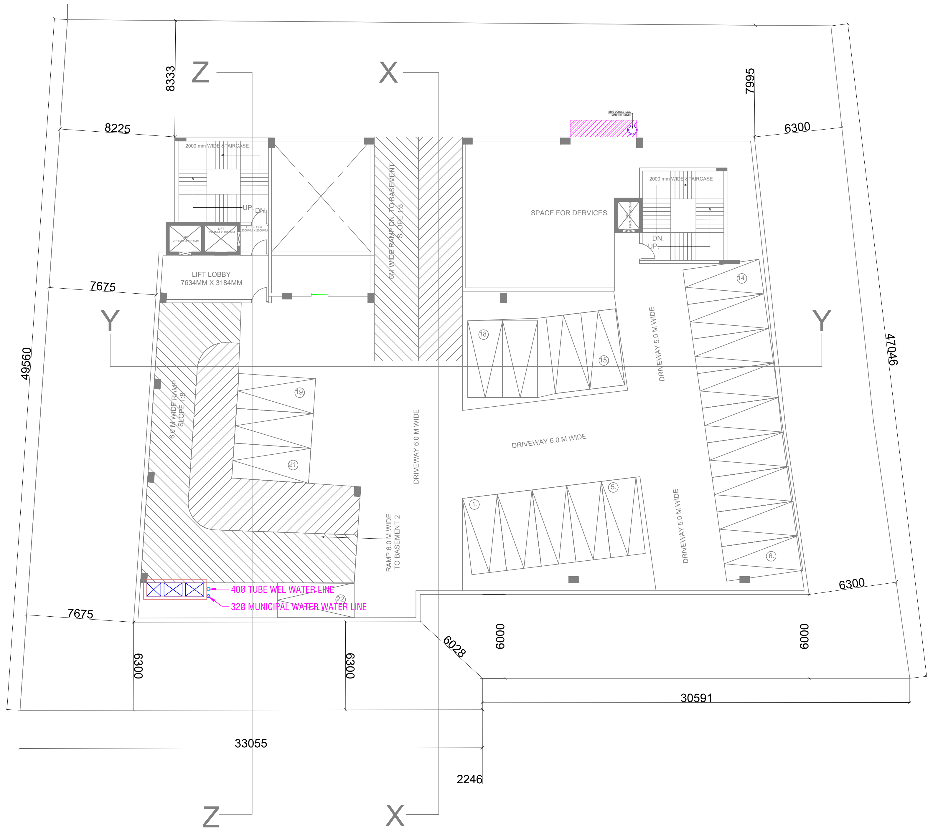
BASEMENT-1 FLOOR PLAN
