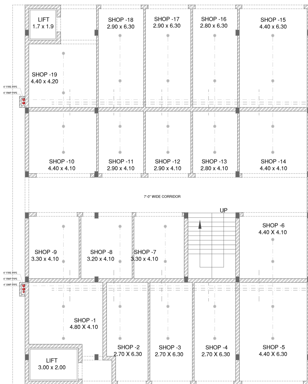
GROUND FLOOR PLAN PLUMBING & FIRE SHAFT PLAN
