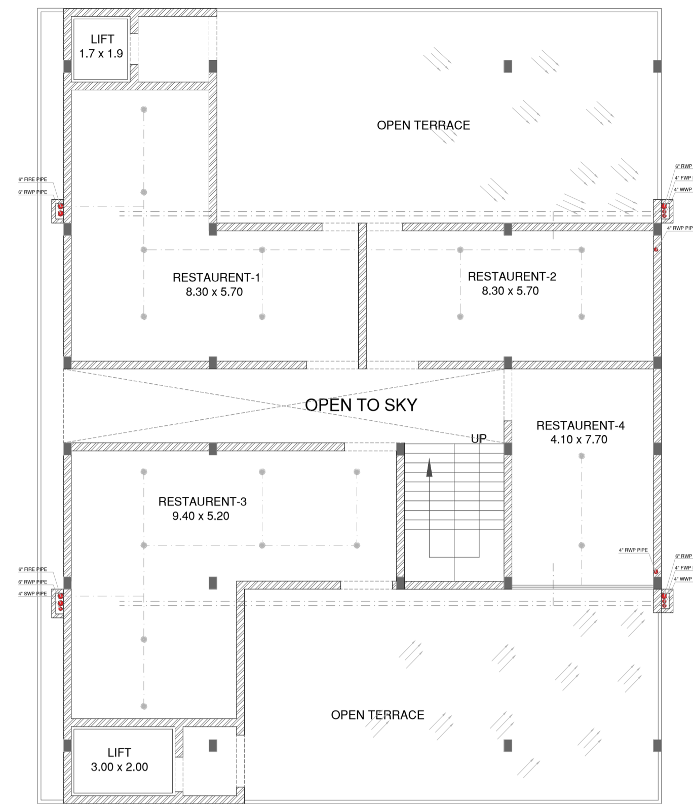
THIRD FLOOR PLAN PLUMBING & FIRE SHAFT PLAN
