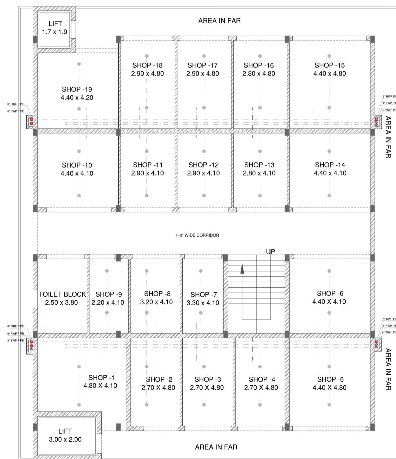
FIRST FLOOR PLAN PLUMBING & FIRE SHAFT PLAN
