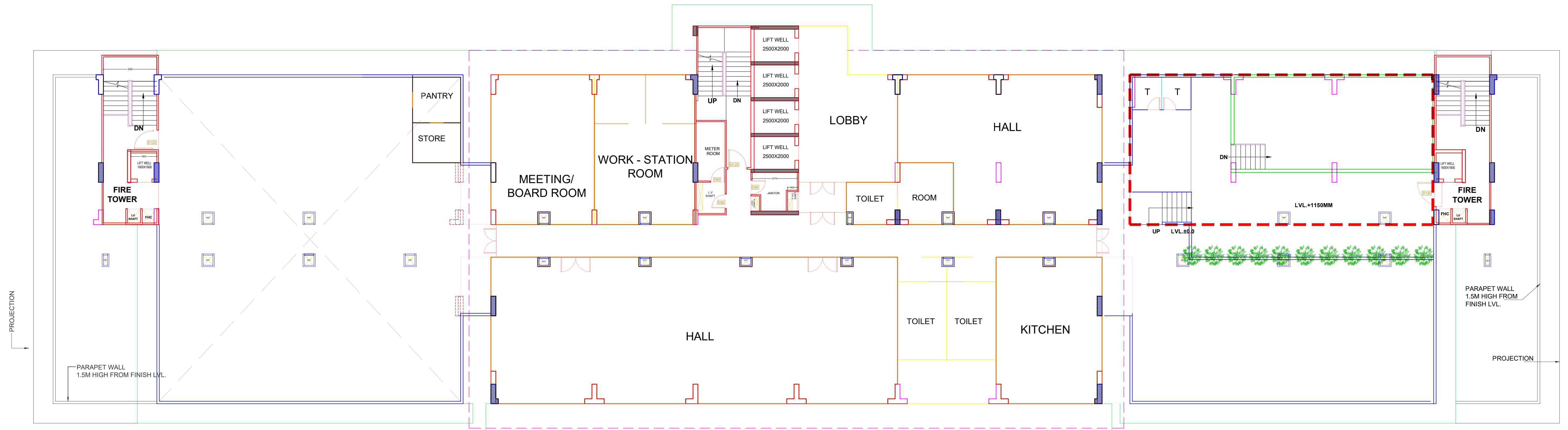
17th FLOOR PLAN
