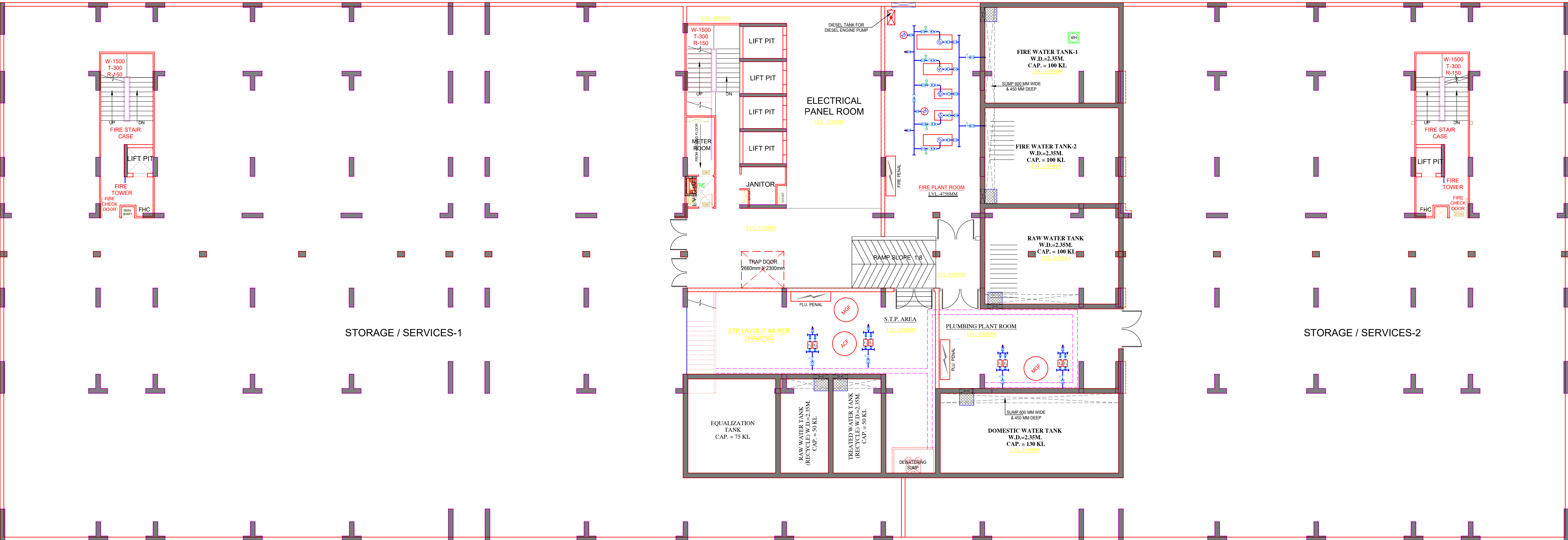
BASEMENT FLOOR PLAN
