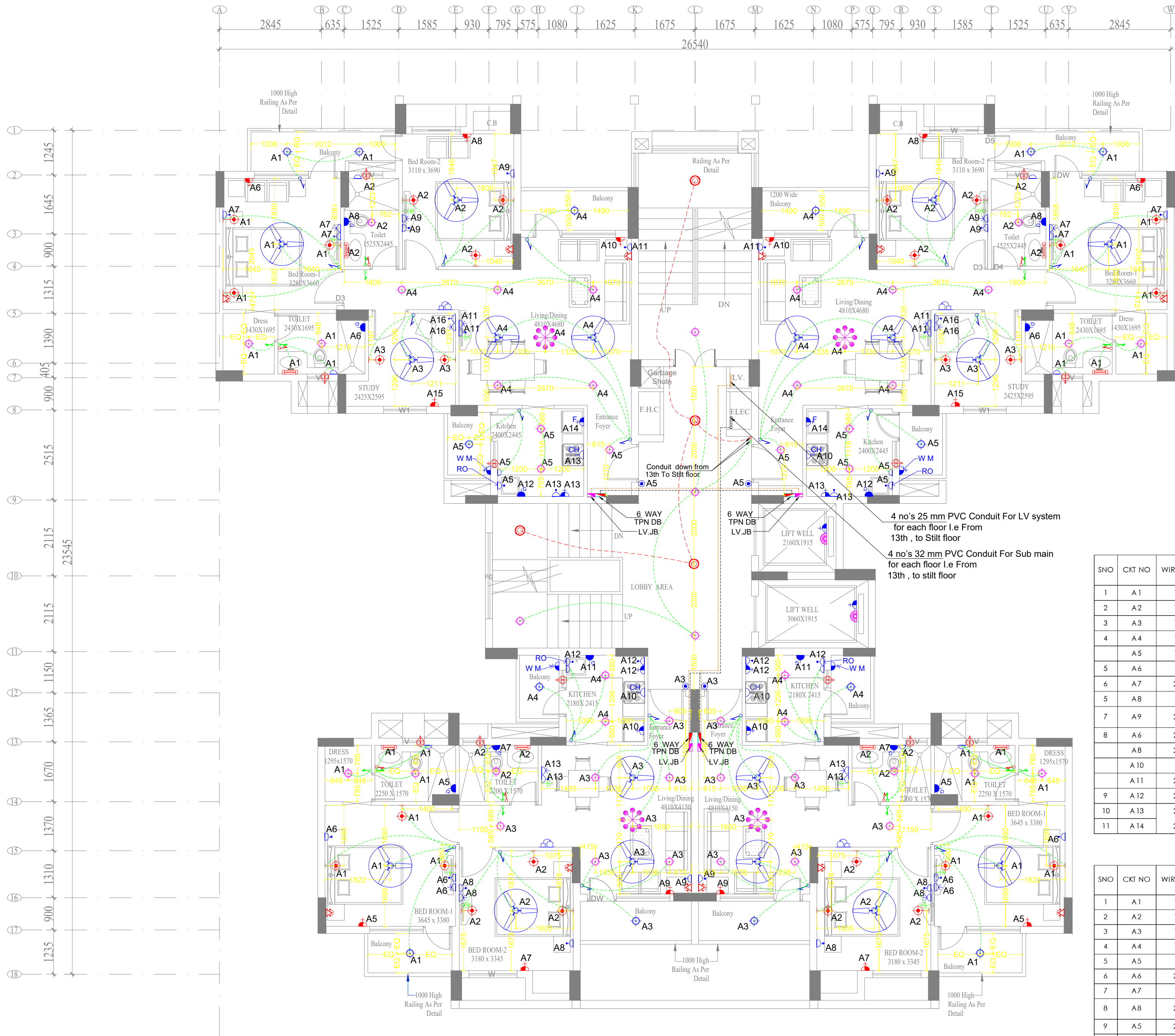
TYPICAL FLOOR PLAN
