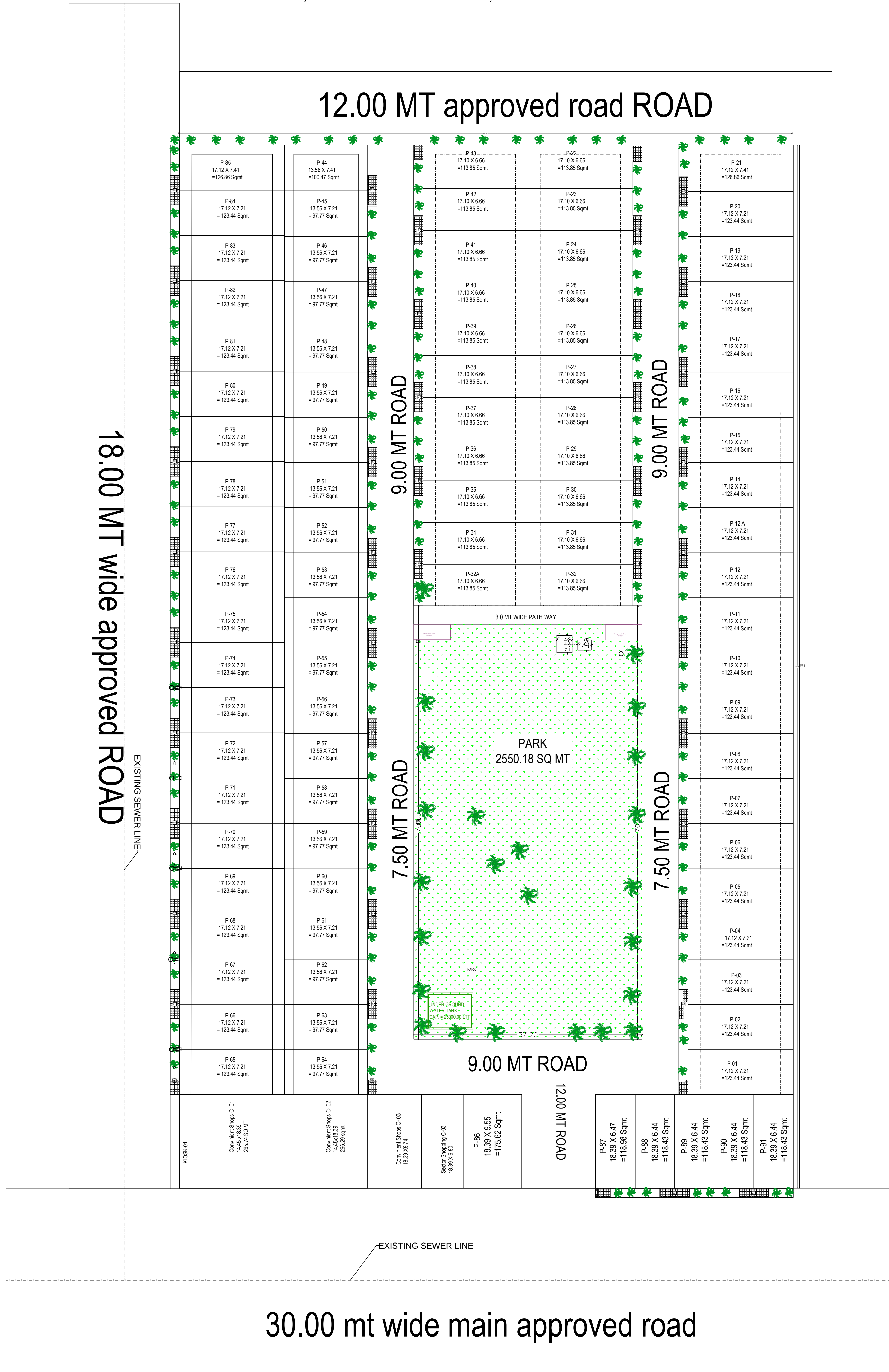
LANDSCAPE- PLAN
