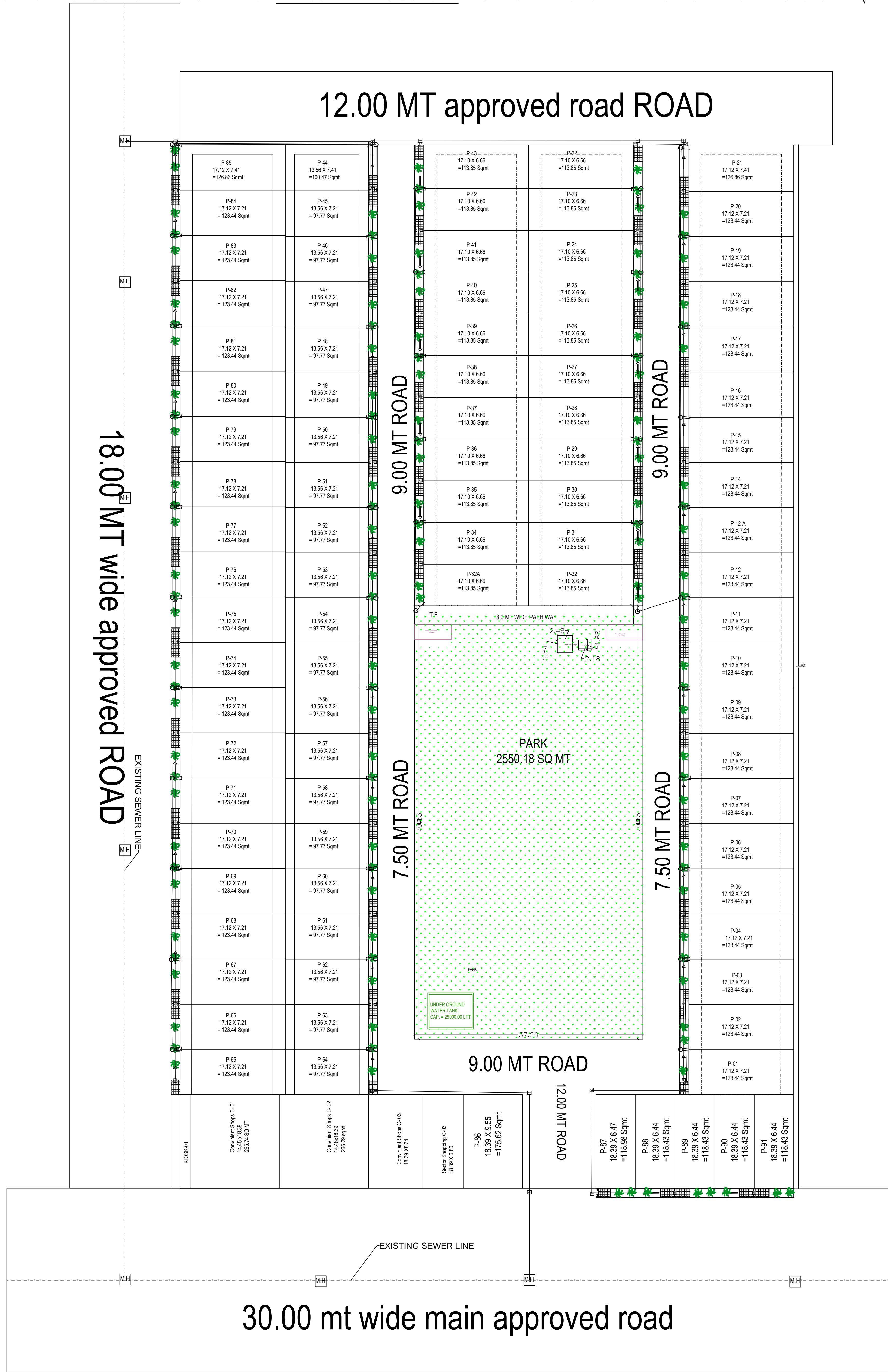
SERVICE PLAN
