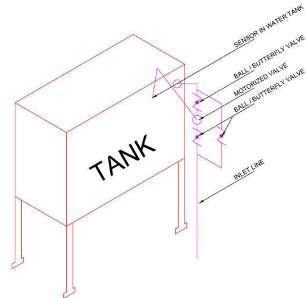
MOTORIZED VALVE DETAIL
