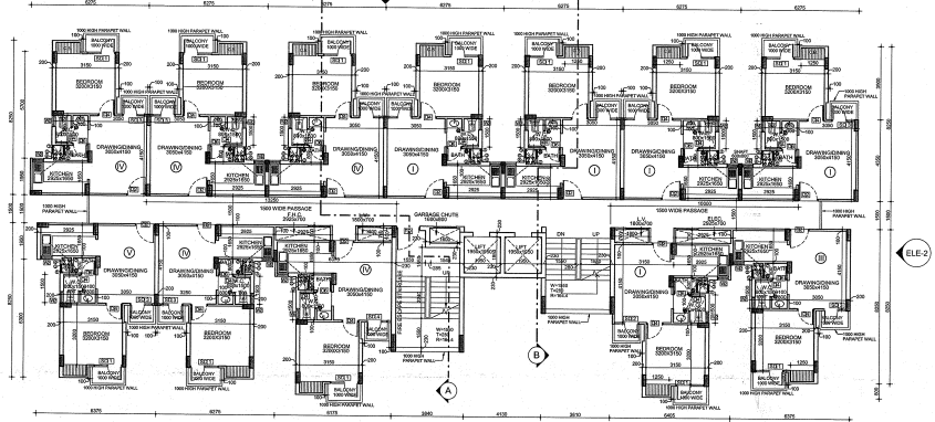
② 9TH FLOOR PLAN 1:100
