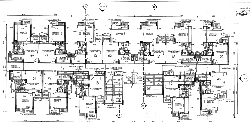
④ 11TH & 12TH FLOOR PLAN 1:100
