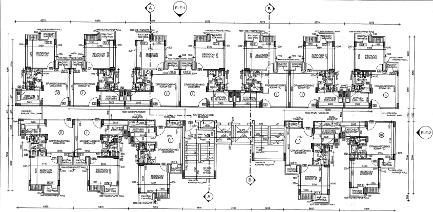
① 6TH TO 8TH FLOOR PLAN 1:100
