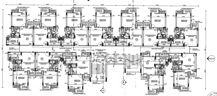
⑤ 13TH FLOOR PLAN 1:100
